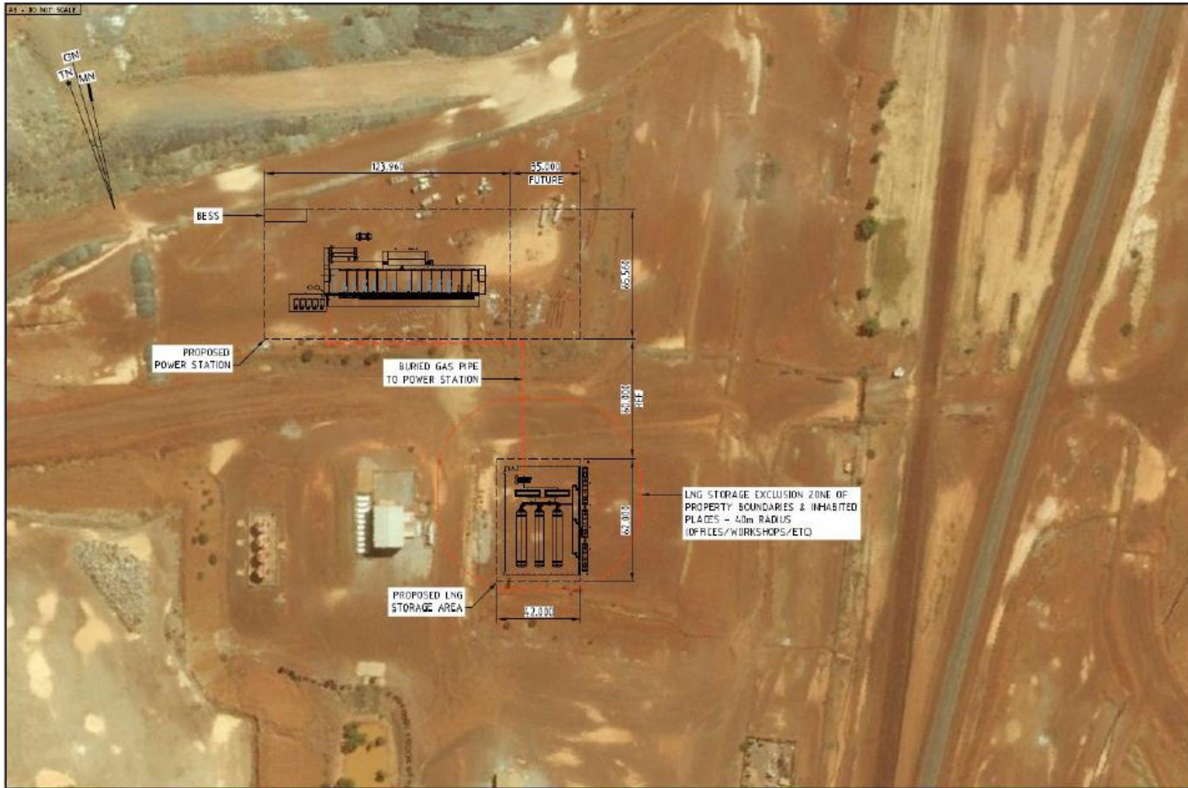
Figure 22: Hybrid Power Generation Facility (Bluebird Power Station) and LNG Storage Area Layout
