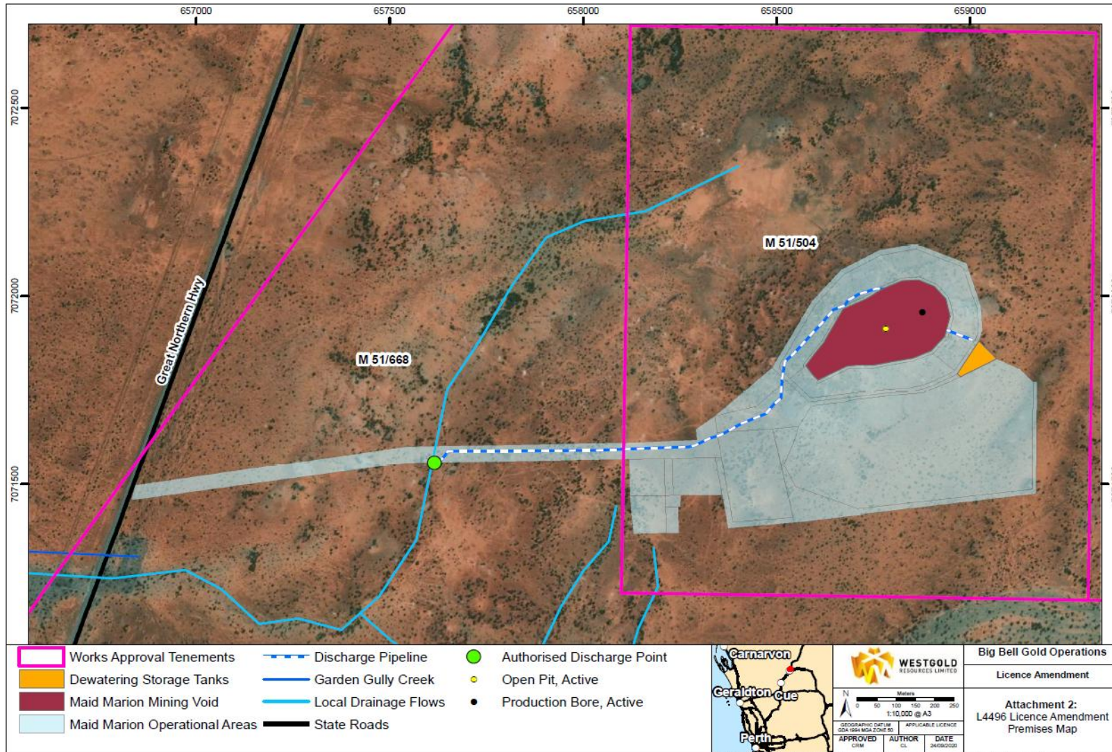
Figure 19: Maid Marion Dewatering Infrastructure and Discharge Point
