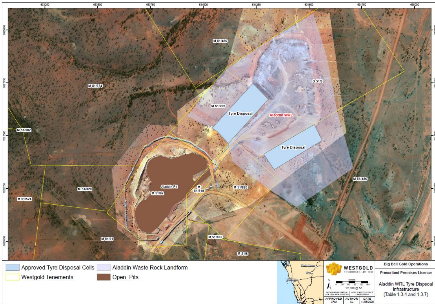
Figure 12: Aladdin WRL and Tyre Disposal Infrastructure
