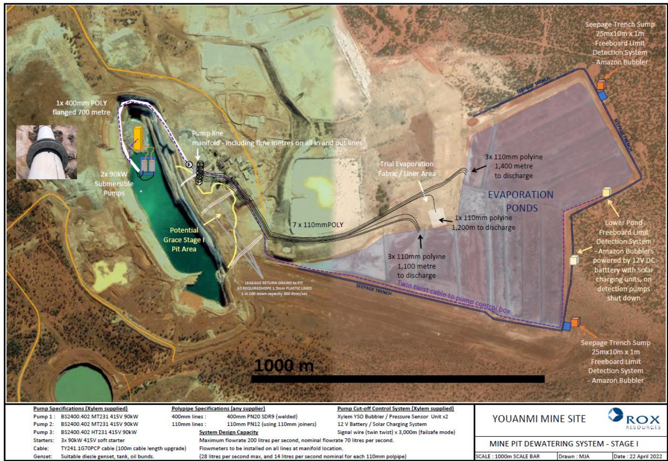
Figure 4: Map of the Main Pit dewatering infrastructure. Blue squares are seepage collection sump locations.
