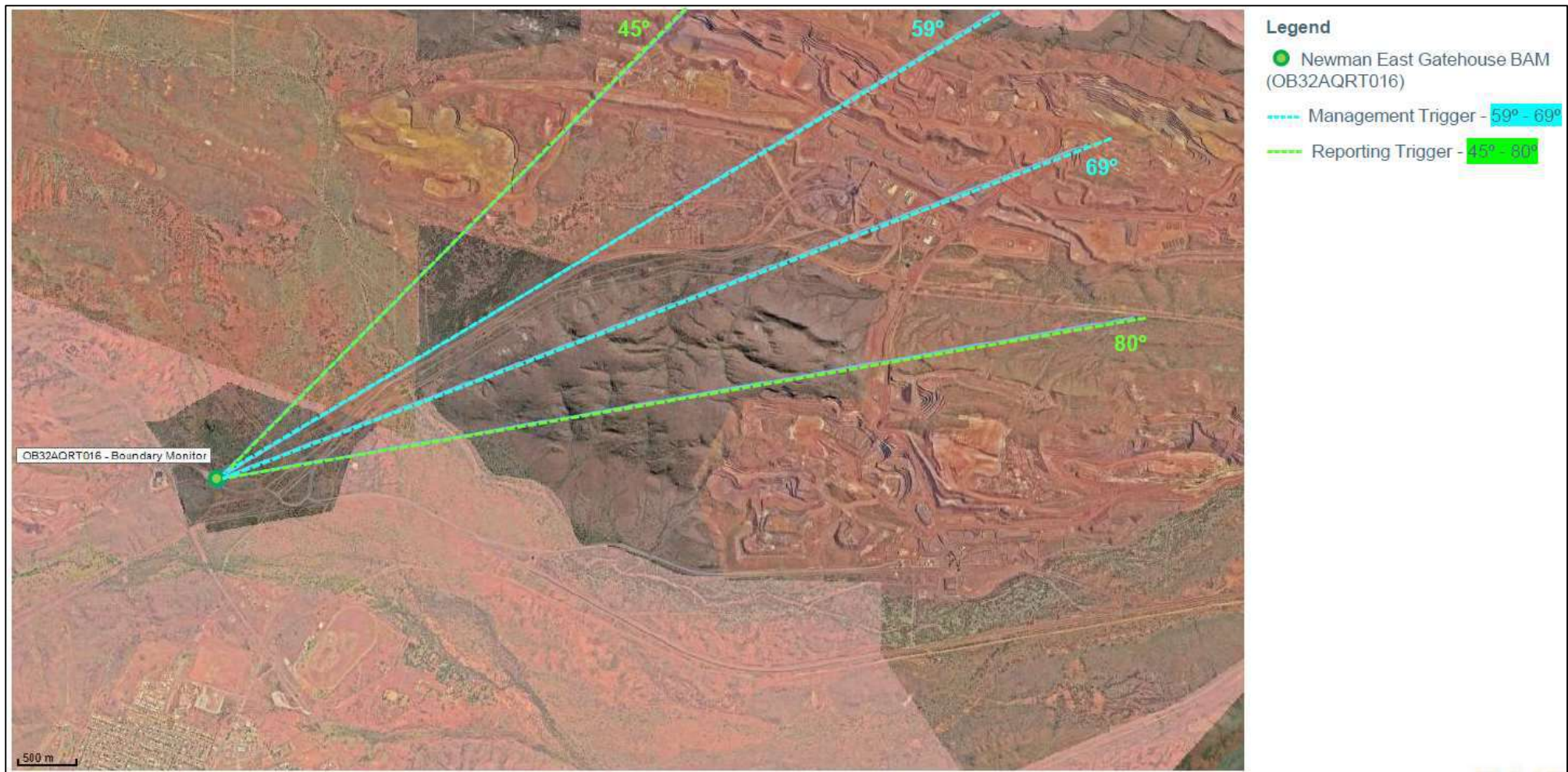
Figure 6: Management trigger wind arcs for boundary monitor
