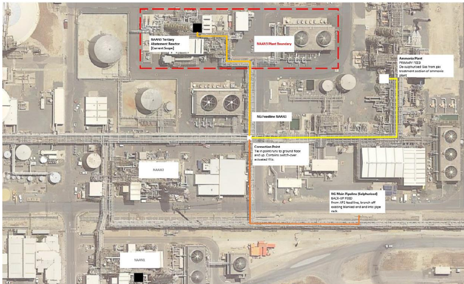
Figure 2: Location of the Nitric Acid Plants (including NAAN 3) and the SCR where the tertiary abatement reactor will be installed
