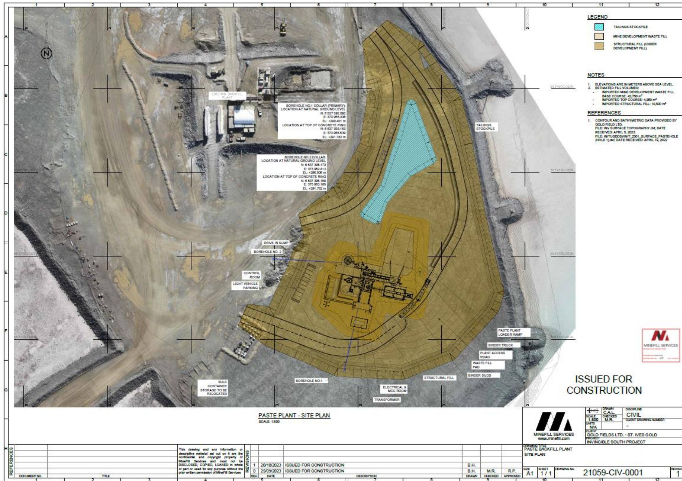
Figure 19: Upgraded Invincible South Paste Plant Layout
