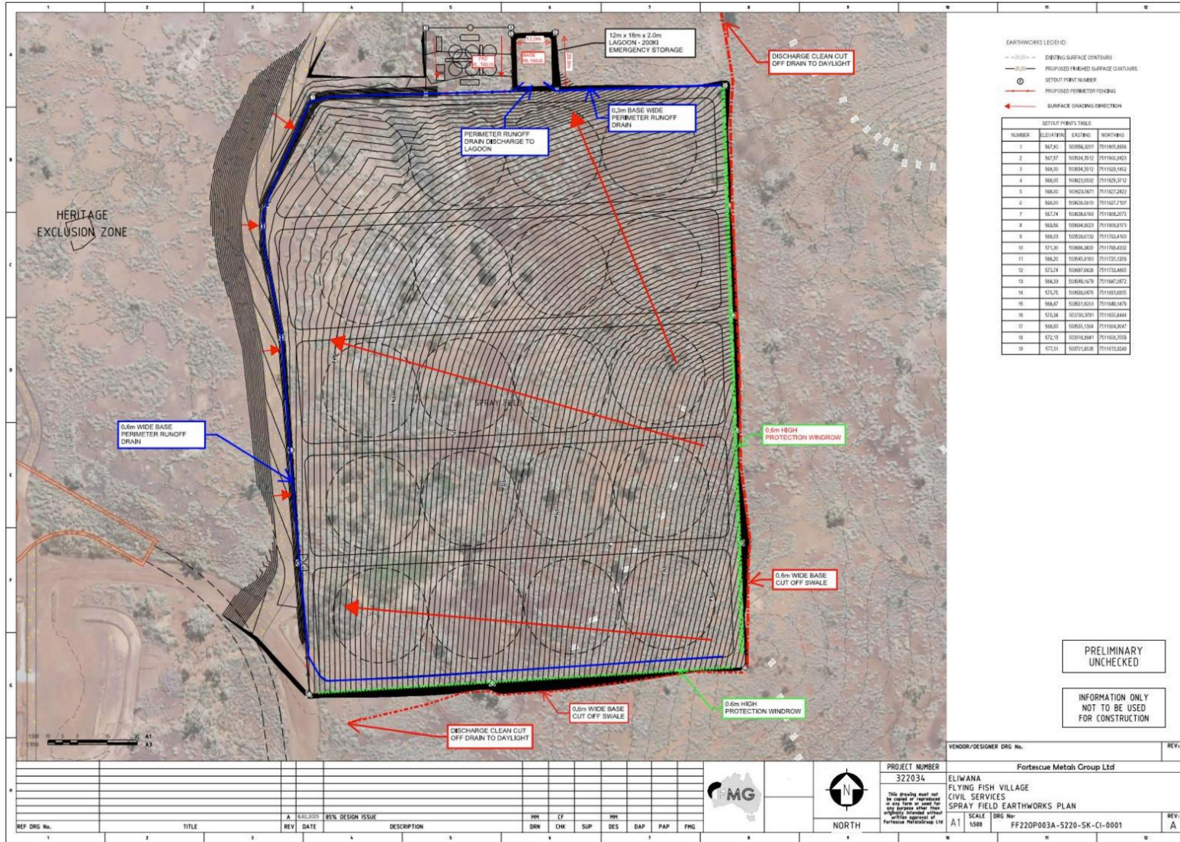
Figure 5: Plan of the irrigation spray field, bunding and drains
