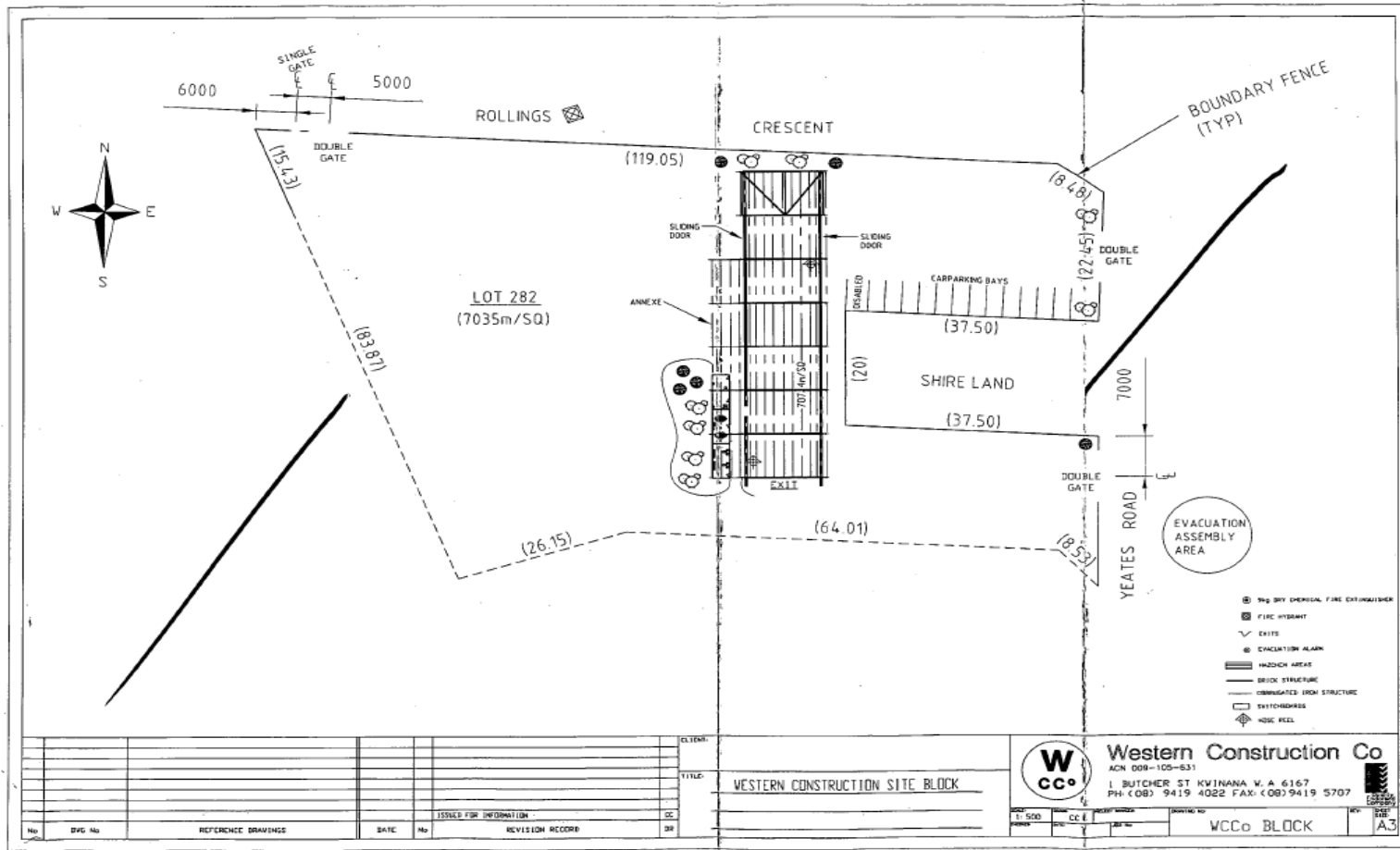
Figure 1: Proposed site layout
