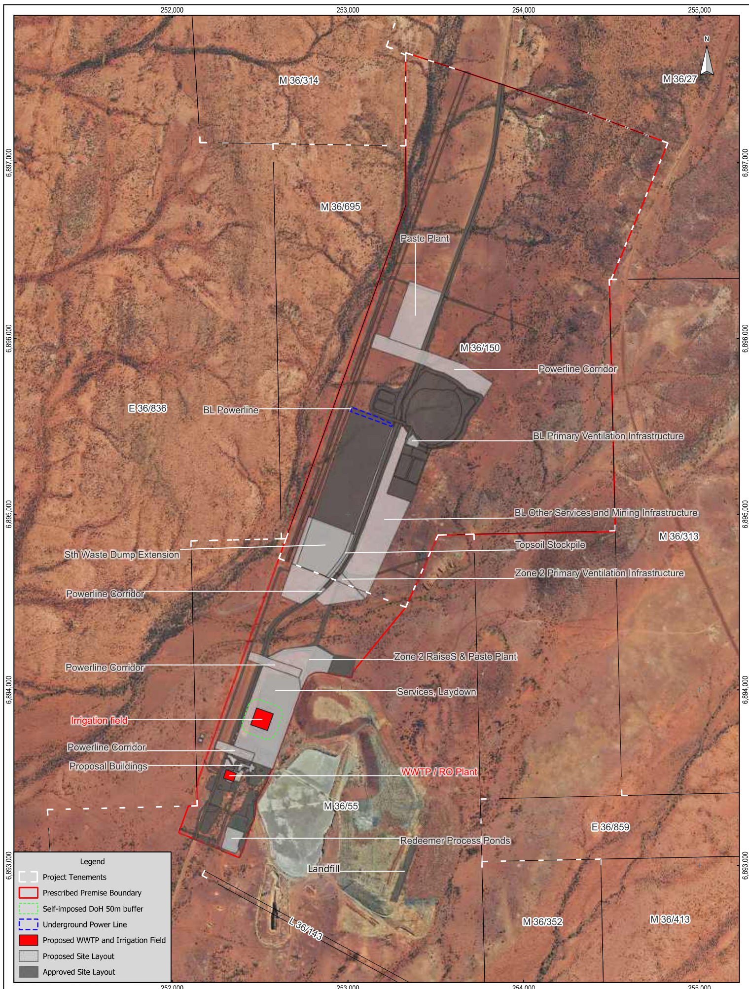
Figure 3 Redeemer/Barren Lands Site Layout
