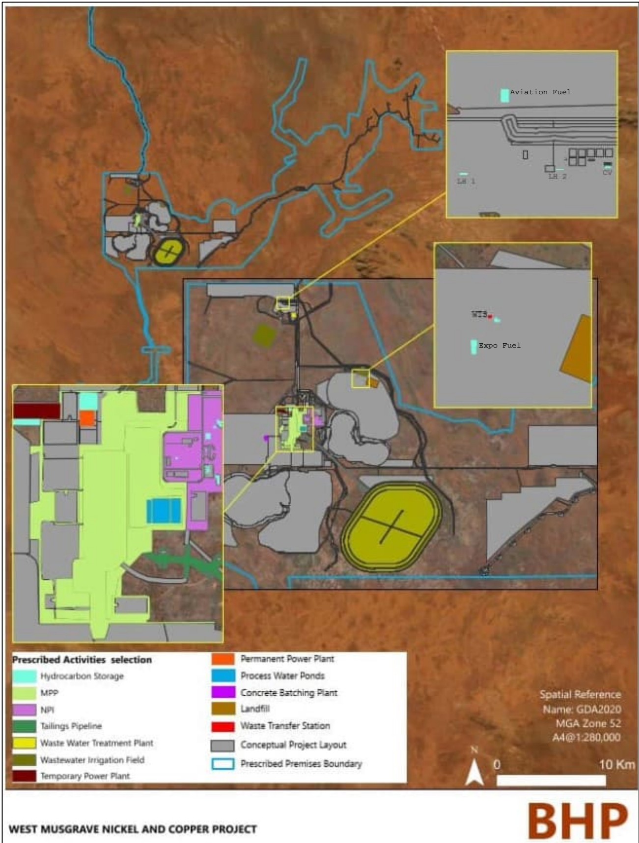
Figure 2-2 Location of Key Physical and Operational Elements
