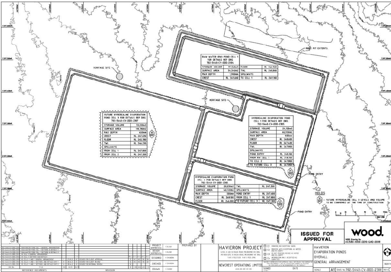
Figure 2: Evaporation Ponds Layout
