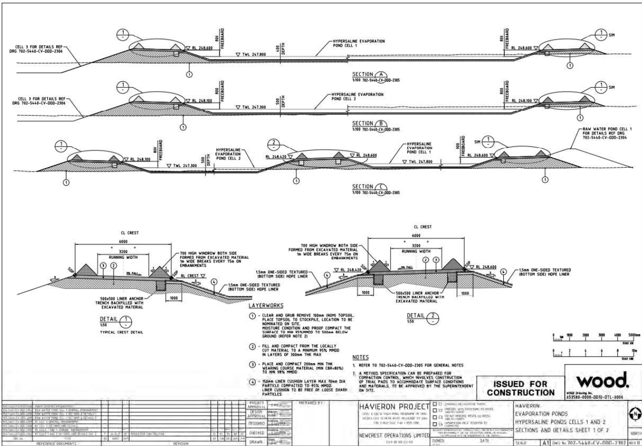
Figure 3: Raw Water Pond cross sections
