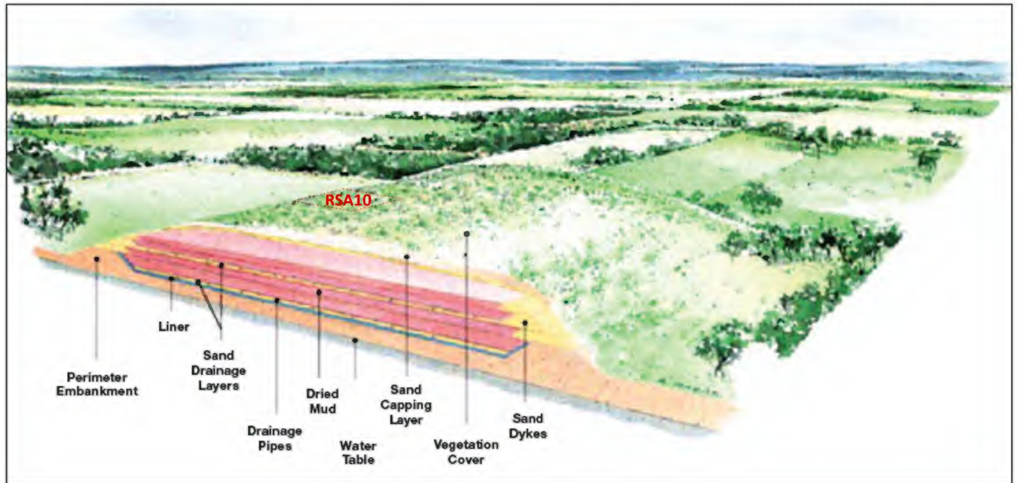
Figure 6: RSA 10 Indicative Closure Landform
