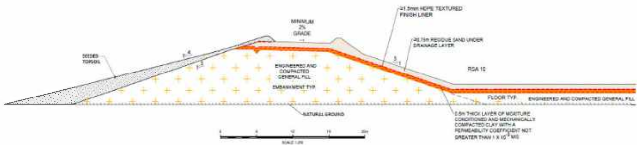
Figure 8: RSA 10 Embankment Wall and Floor Typical Cross Sections
