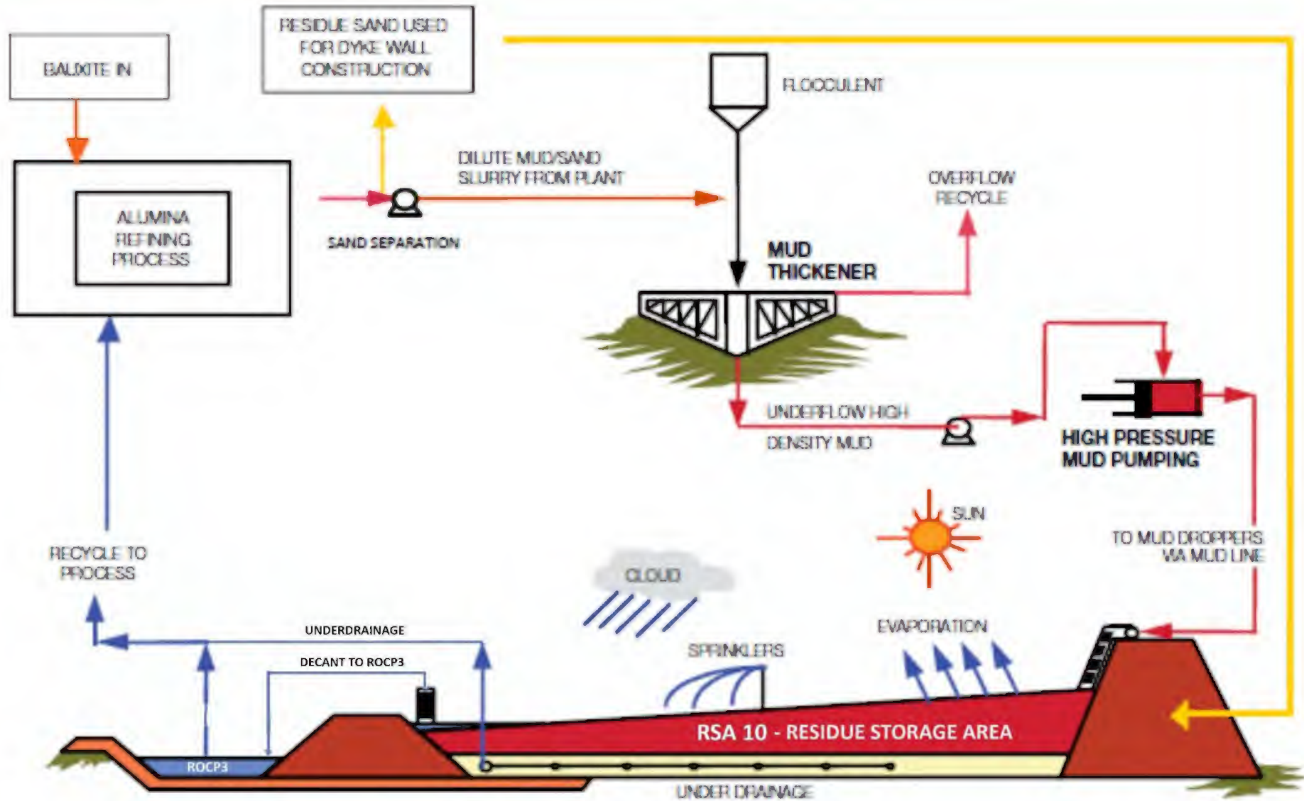
Figure 3: RSA 10 Process Flowchart
