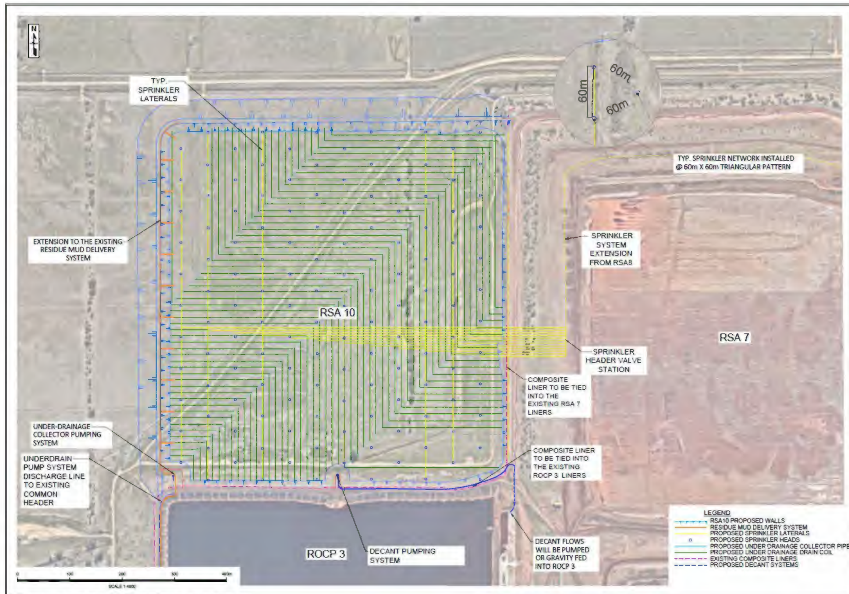
Figure 5: RSA 10 Stage 1 - Construction of RSA 10 Floor and Starter Embankment Walls
