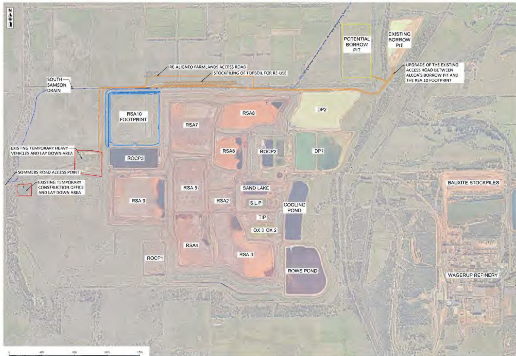
Figure 2: Proposed RSA 10 Infrastructure
