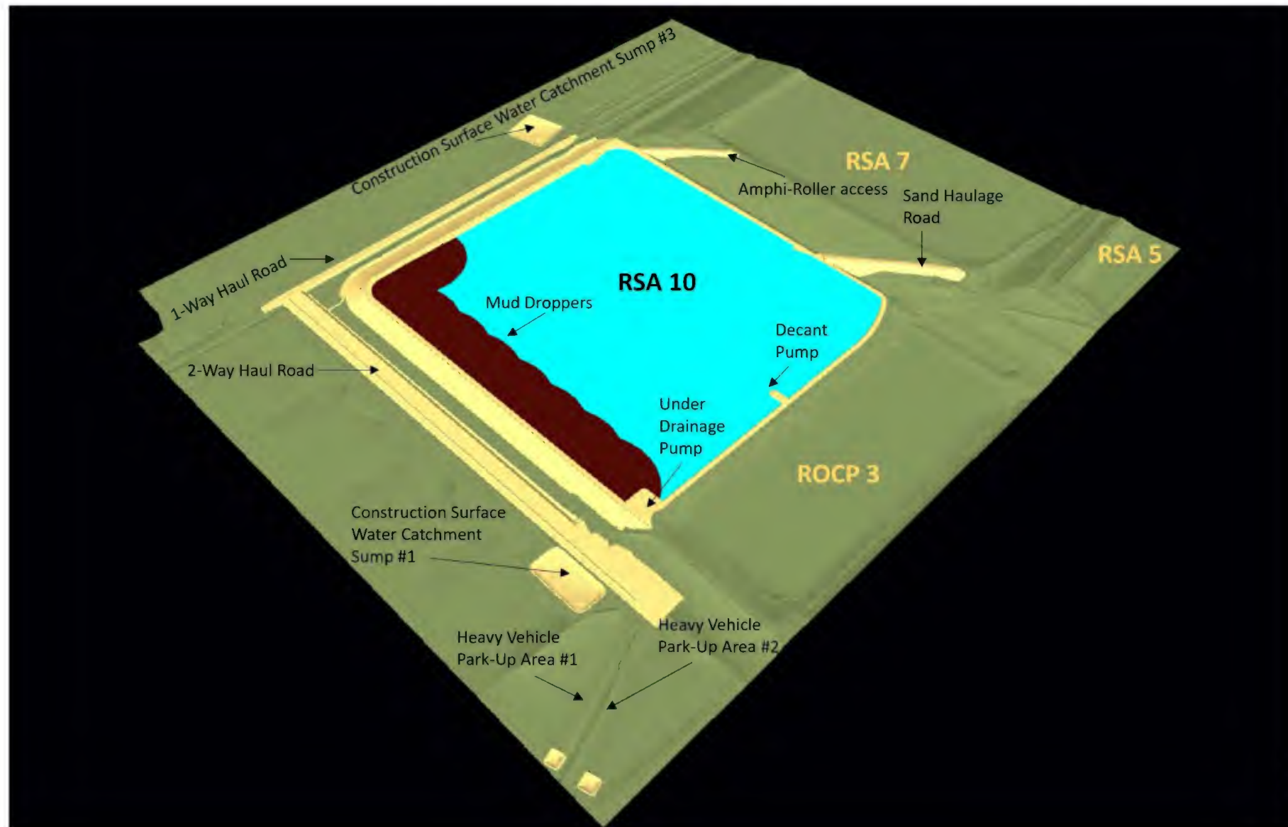
Figure 4: RSA 10 Concept Layout – Starter Embankments Only
