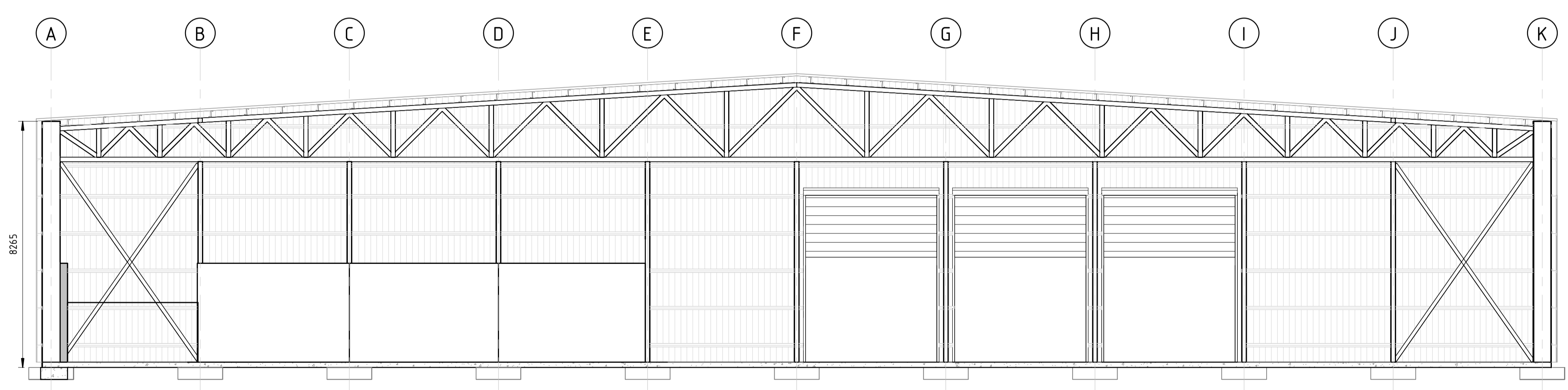
2 SECTION S-105 SCALE 1 : 100
