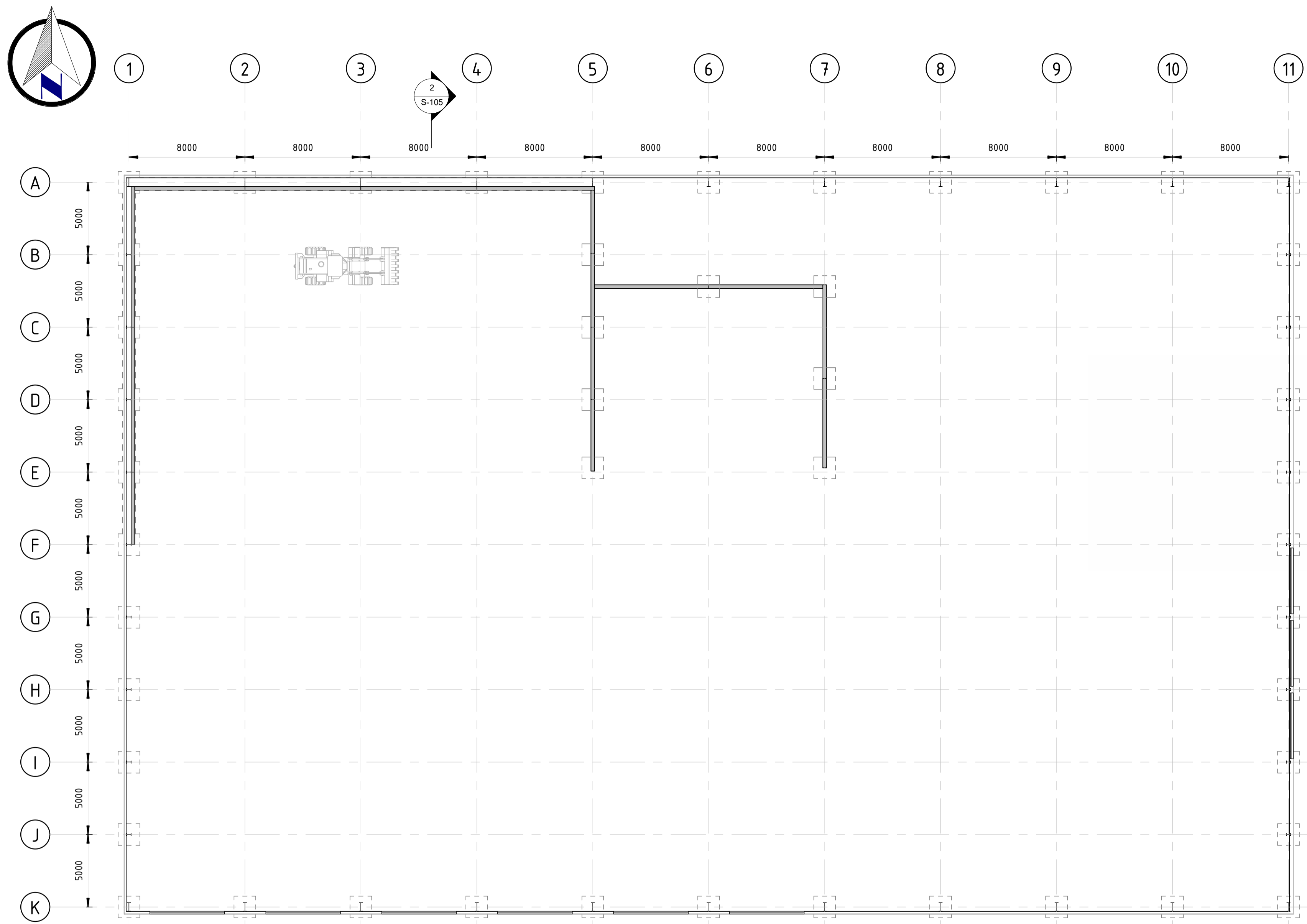
GROUND SLAB LAYOUT 1 : 200
