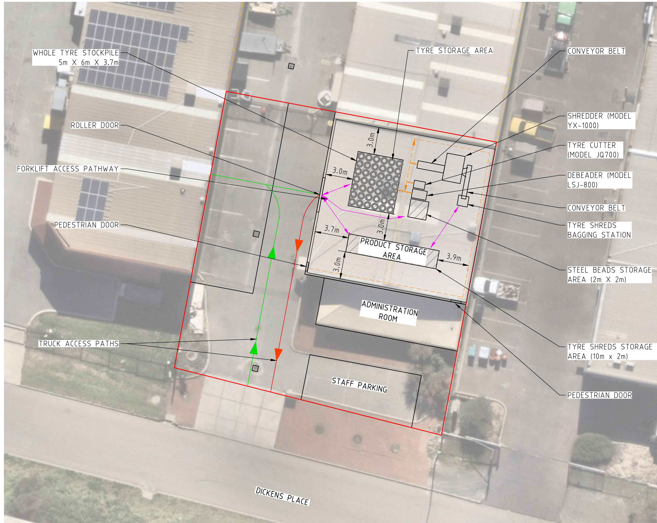
1 PLAN - BUILDING LAYOUT SCALE: 1:250
