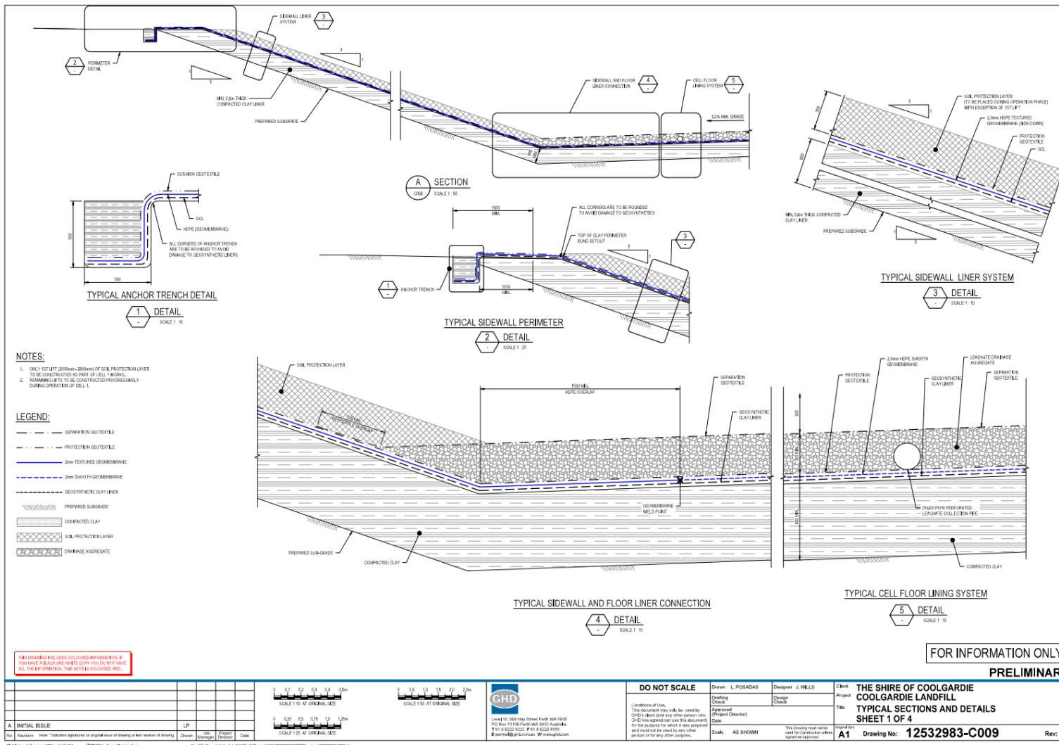
Figure 4: Stage 1 sections and details (1)
