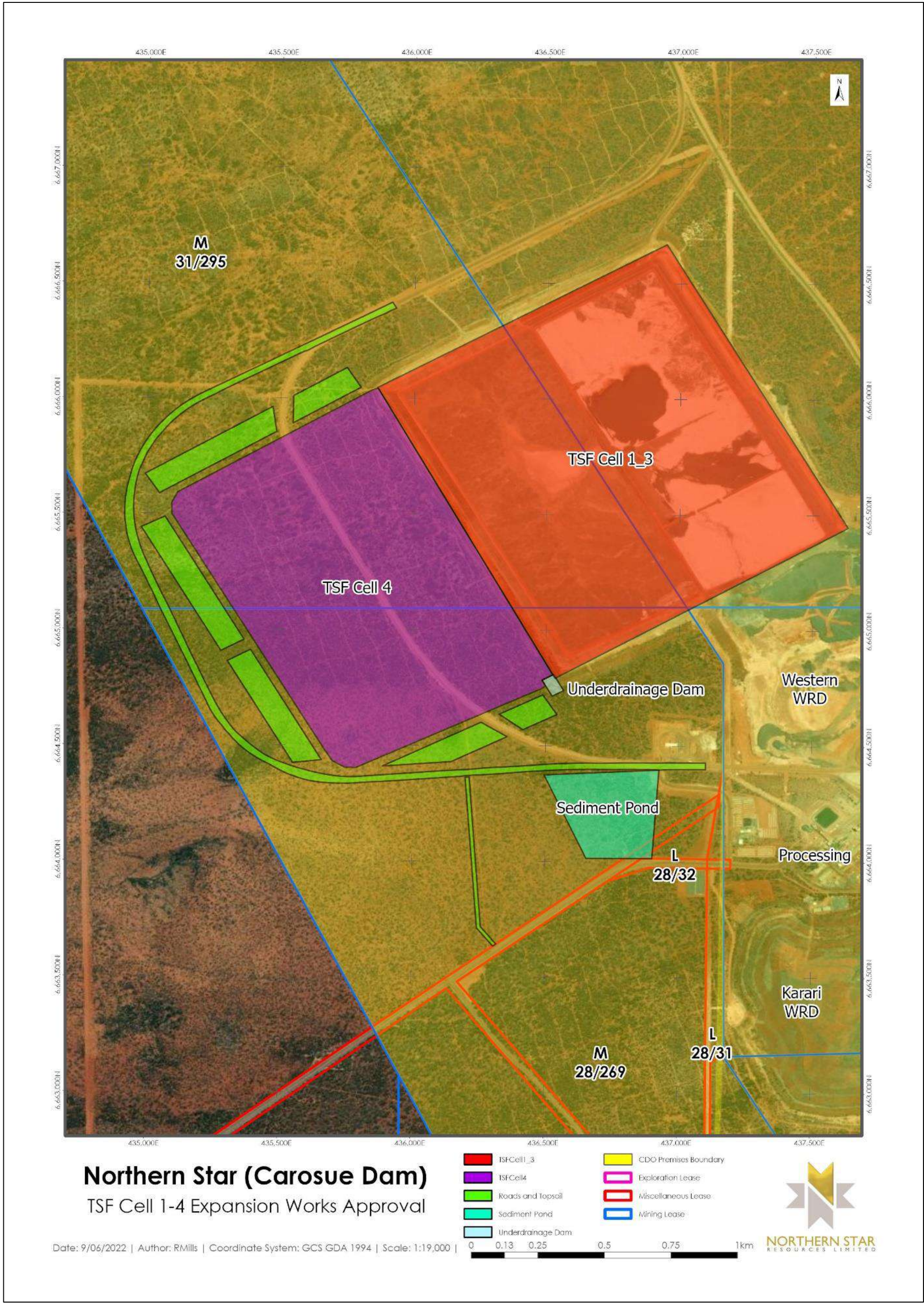
Figure 2: Final TSF and associated Infrastructure layout
