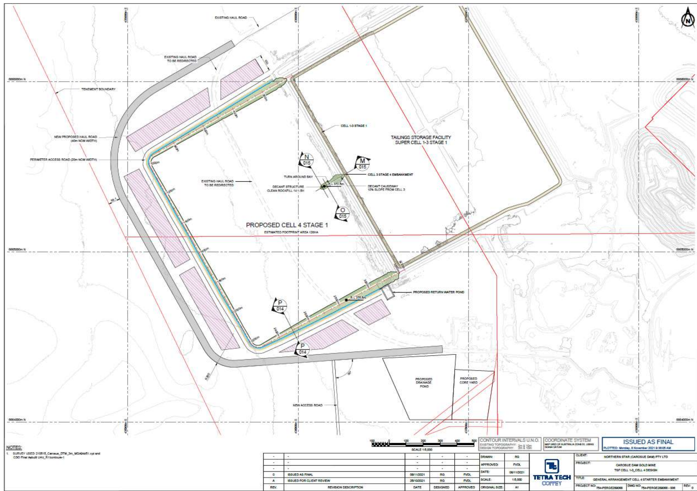
Figure 4: Cell 4 starter embankment
