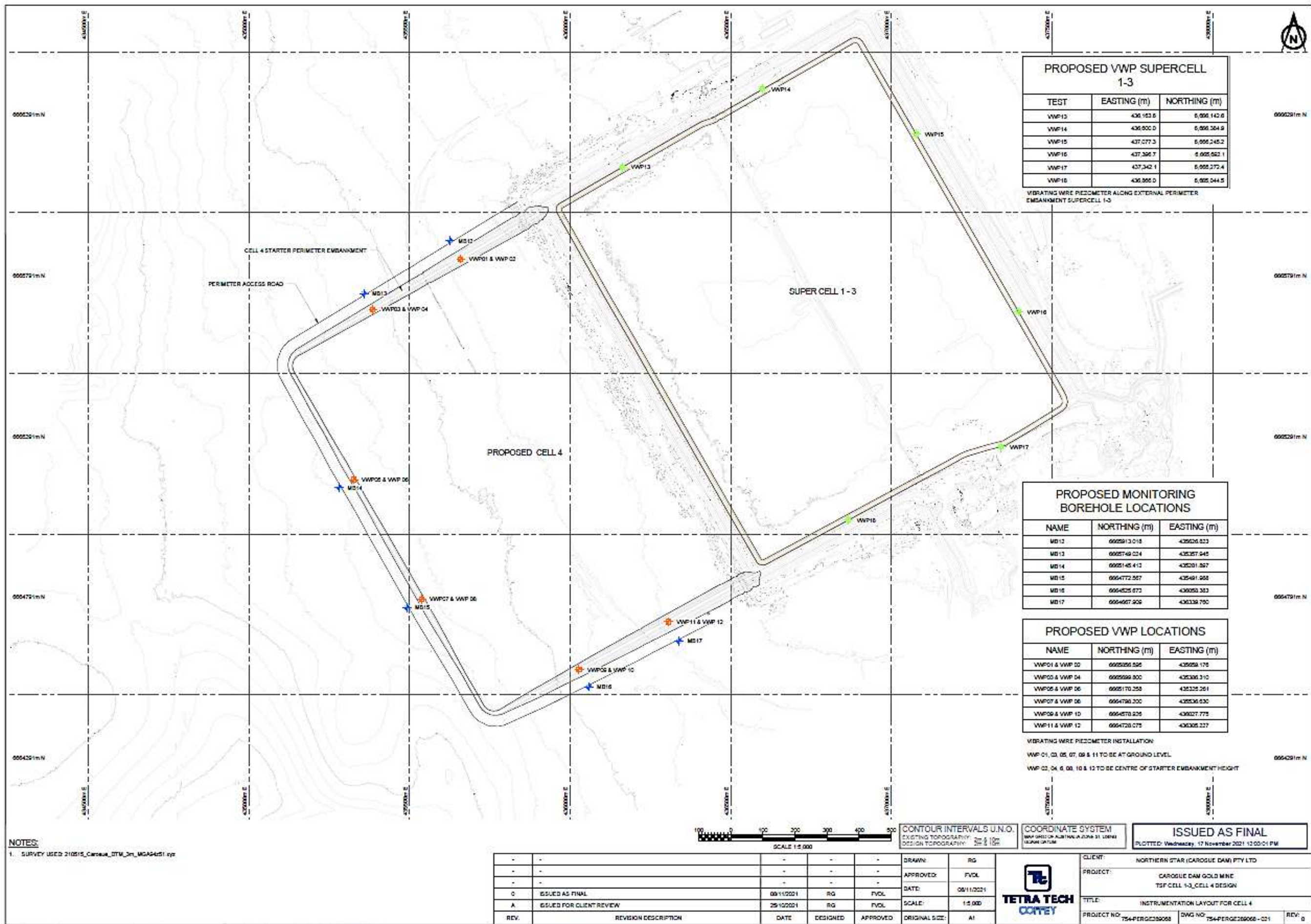
Figure 9: Cell 4 new bores and piezometer positions
