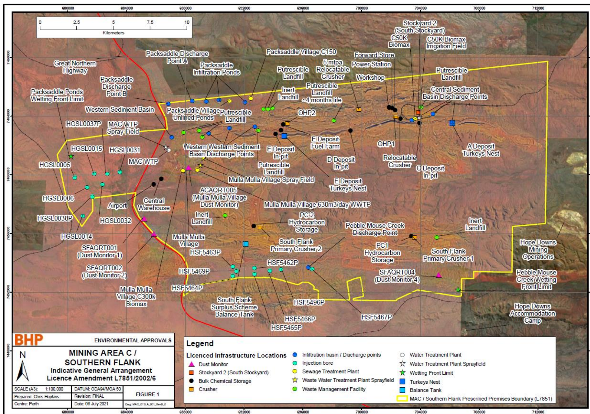
Figure 1: Site Layout and Prescribed Premises Boundary
