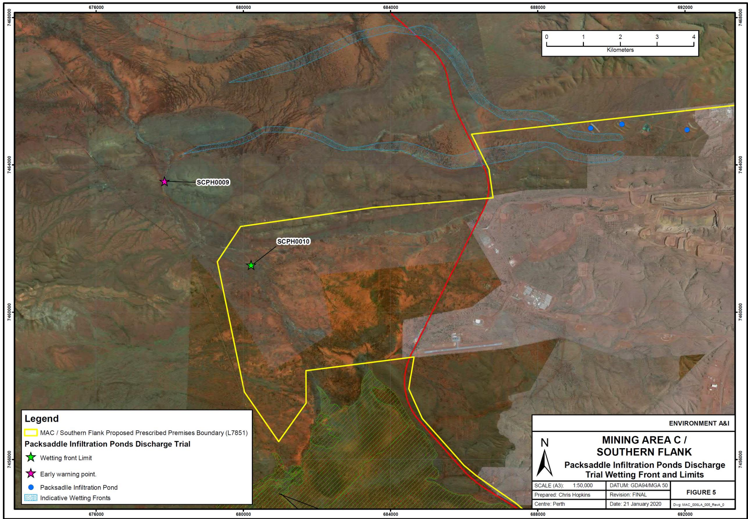
Figure 4: Packsaddle Infiltration Ponds Discharge Trial Wetting Front and Limit
