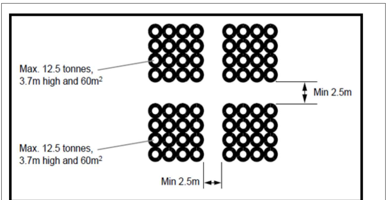
Figure 6: Minimum Separation Distance Between Piles.
