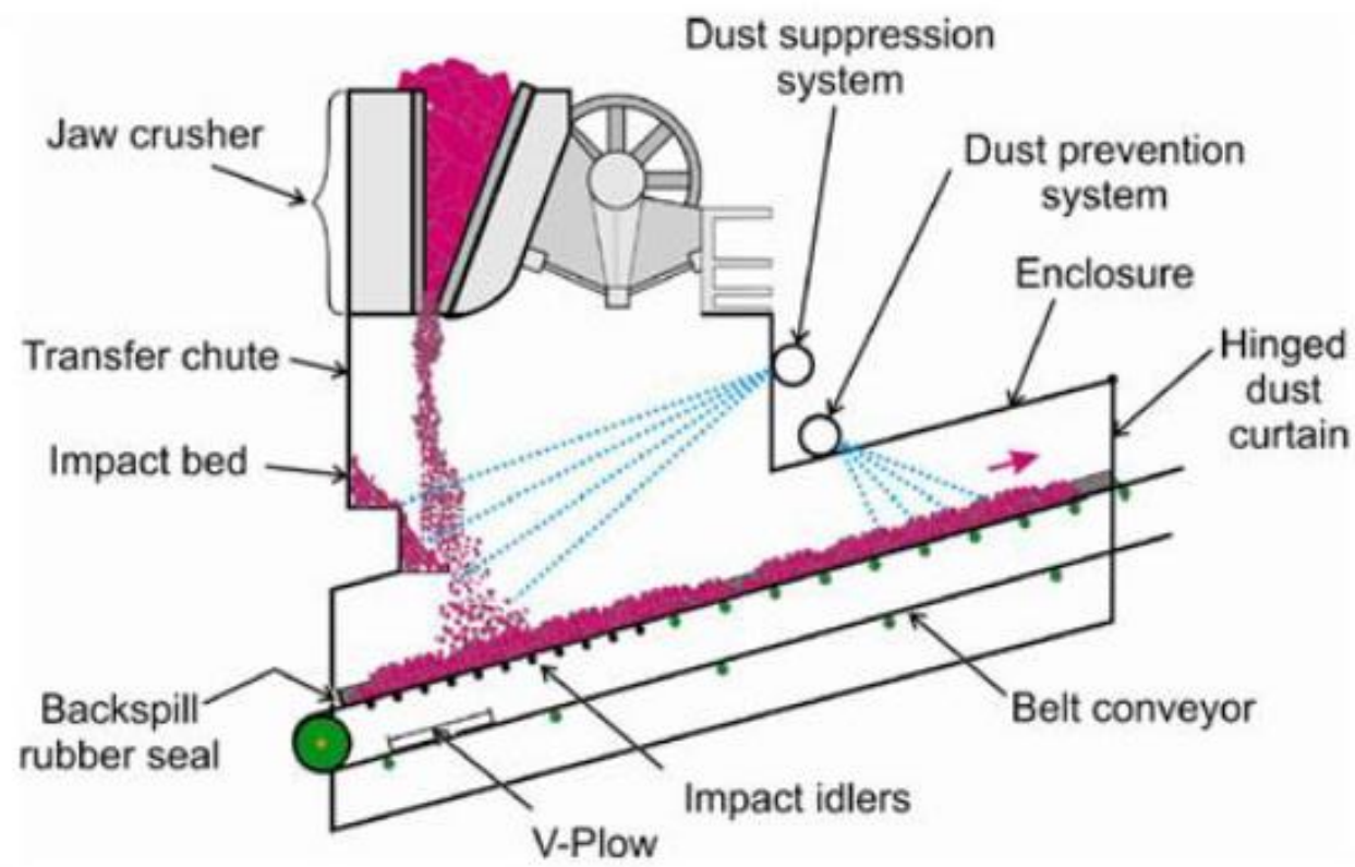
Figure 3: Conceptual map of crushing screening plant
