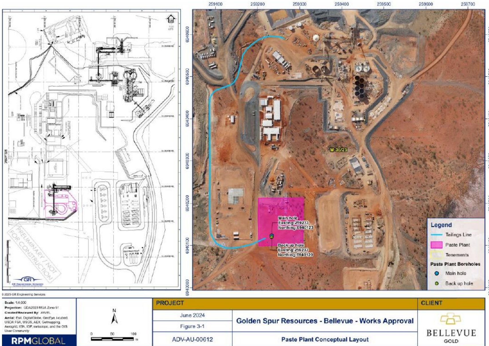
Figure 3: Location of paste plant, paste plant boreholes, and return water and tailings pipelines.
