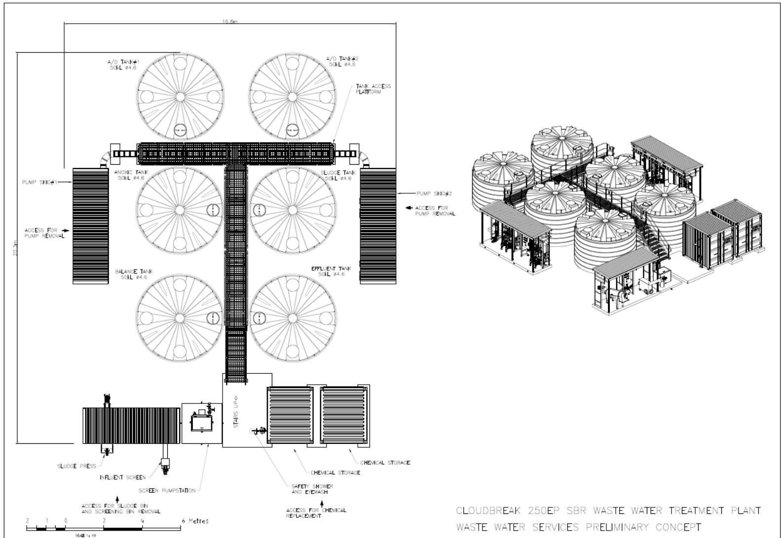
Figure 18: Cloudbreak 250EP SBR Wastewater Treatment Plant Wastewater Services Preliminary Concept
