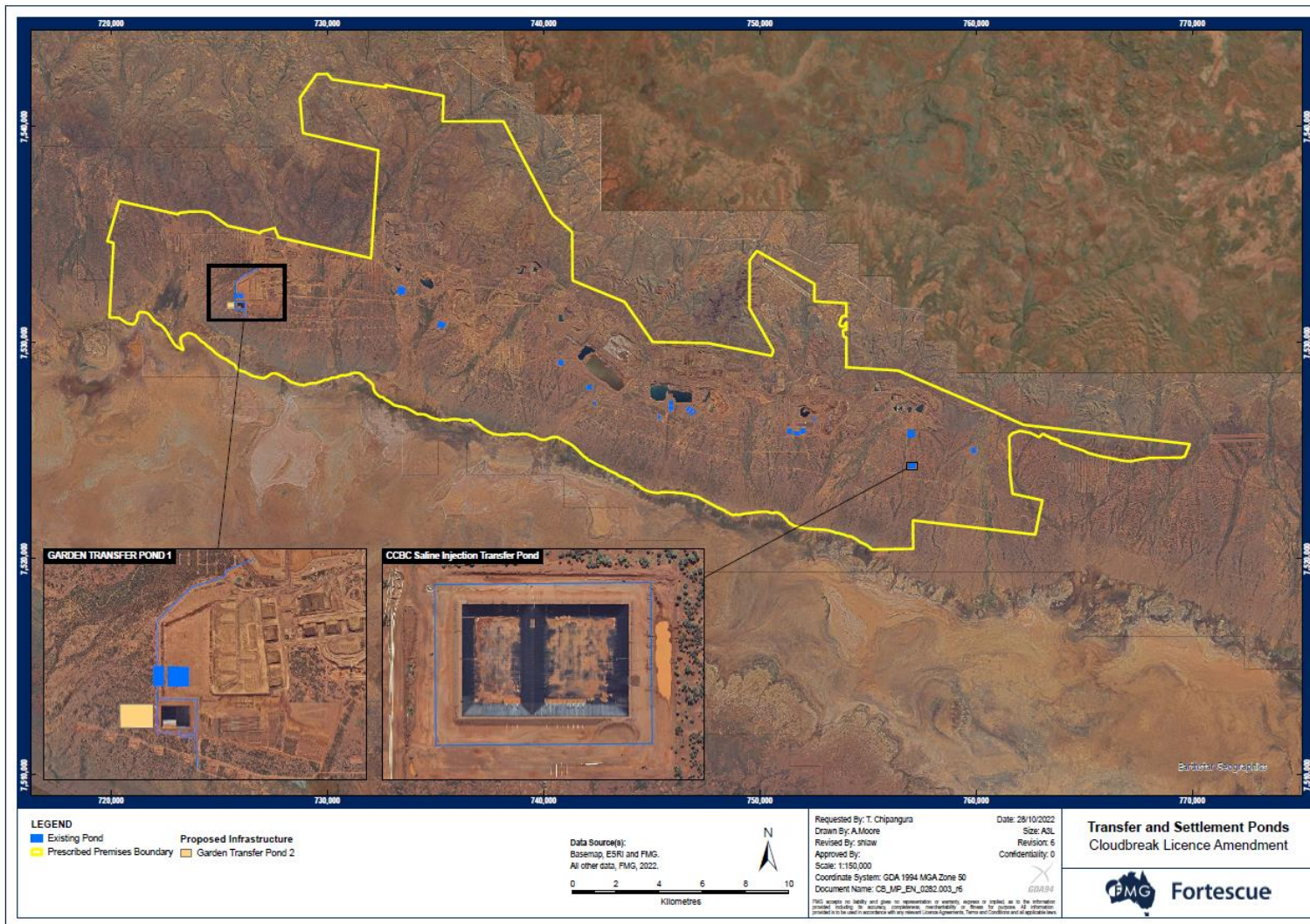
Figure 16: Location of the Garden Transfer Pond 1 and CCBC Saline Injection Transfer Pond containment infrastructure defined in Condition 2, Table 1
