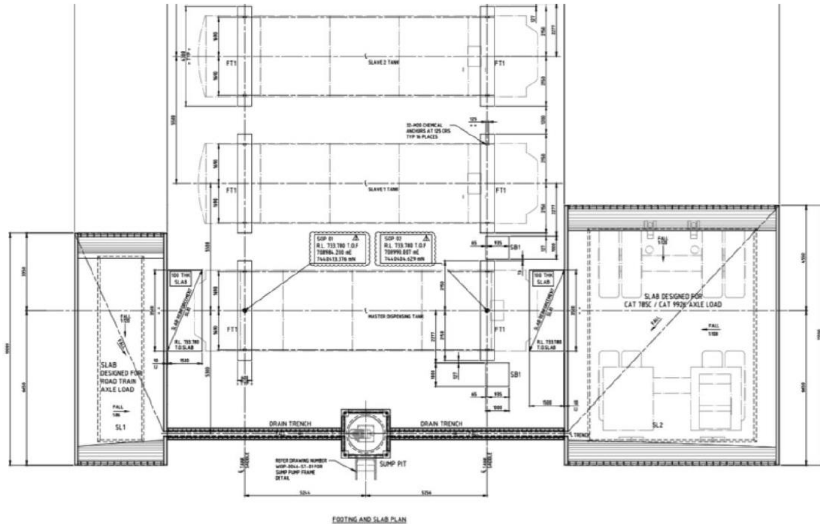
Figure 15: Layout of Upper Cane Bulk Fuel Farm
