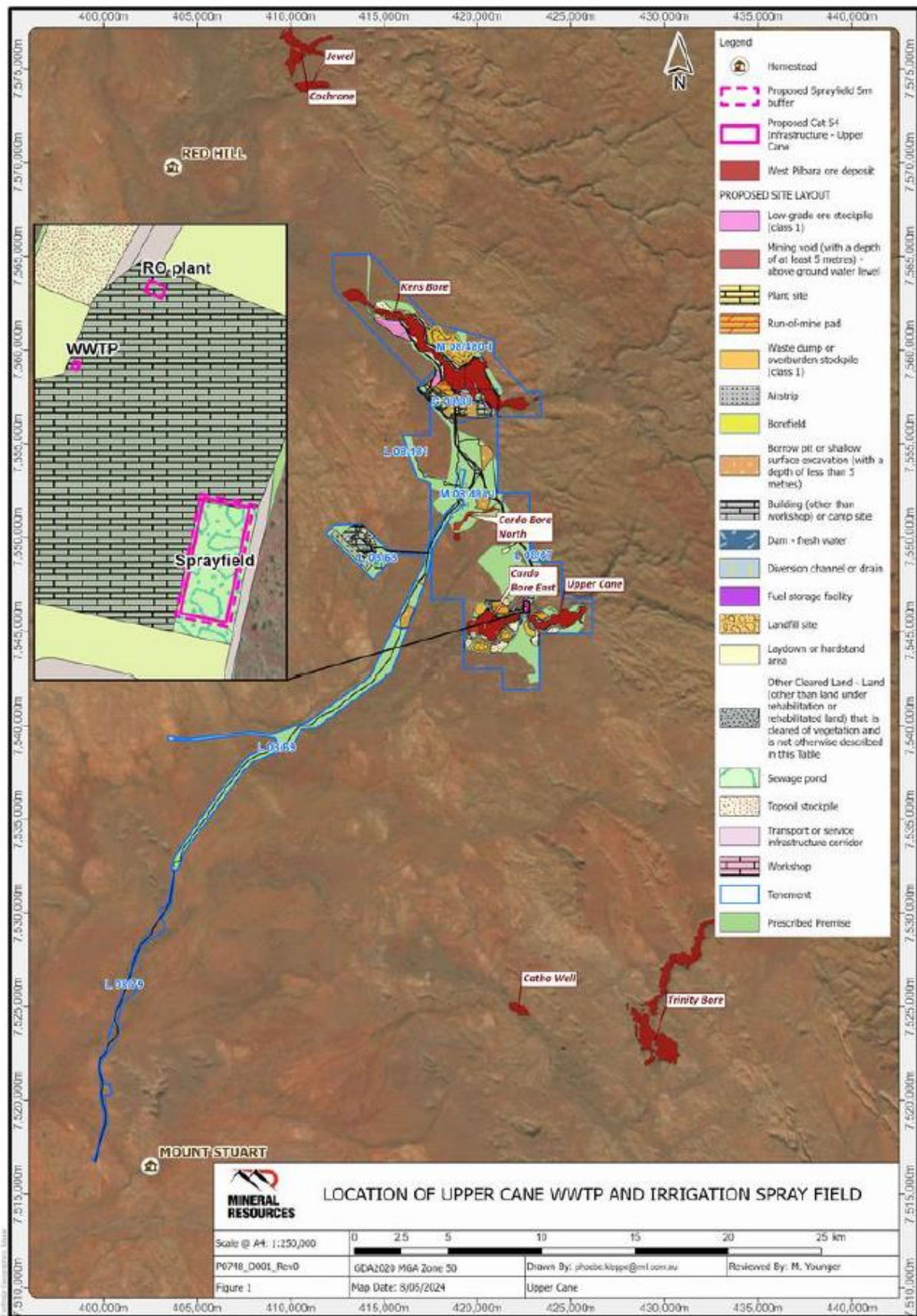
Figure 11: Location of the Upper Cane WWT and Irrigation Spray Field
