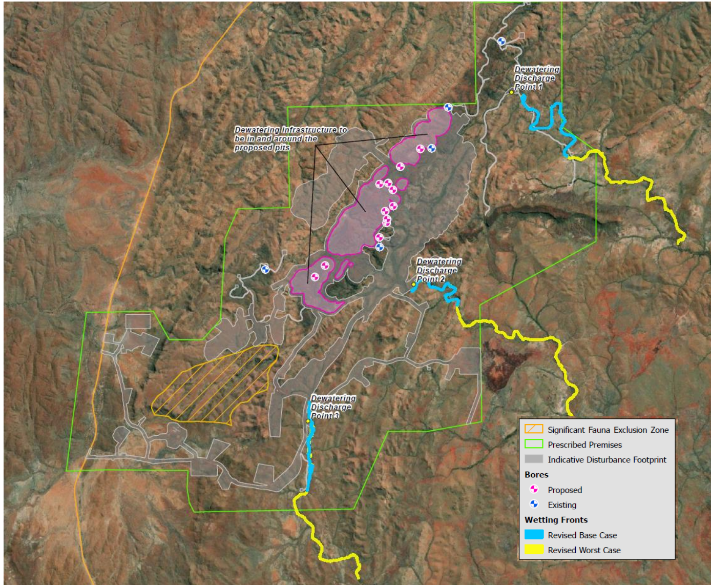
Figure 5 Dewatering infrastructure approximate location
