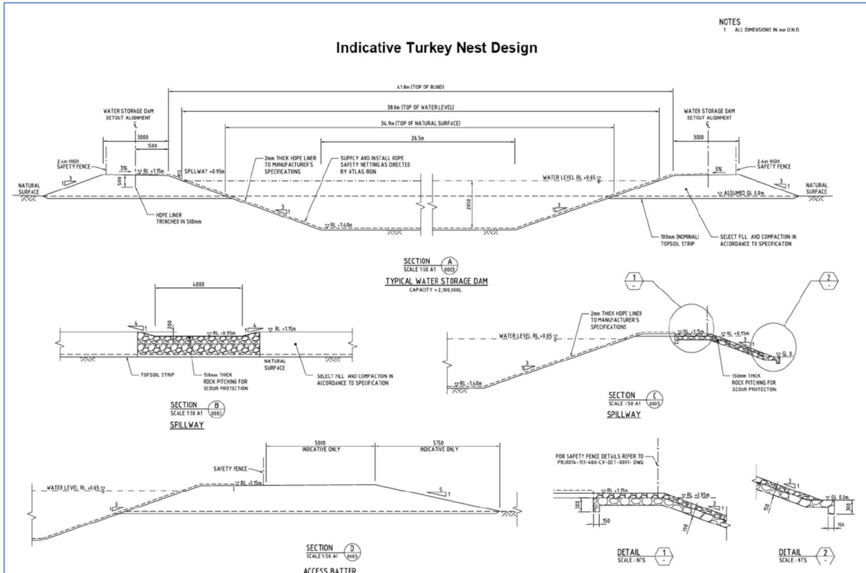
Figure 13 Indicative turkey's nest design
