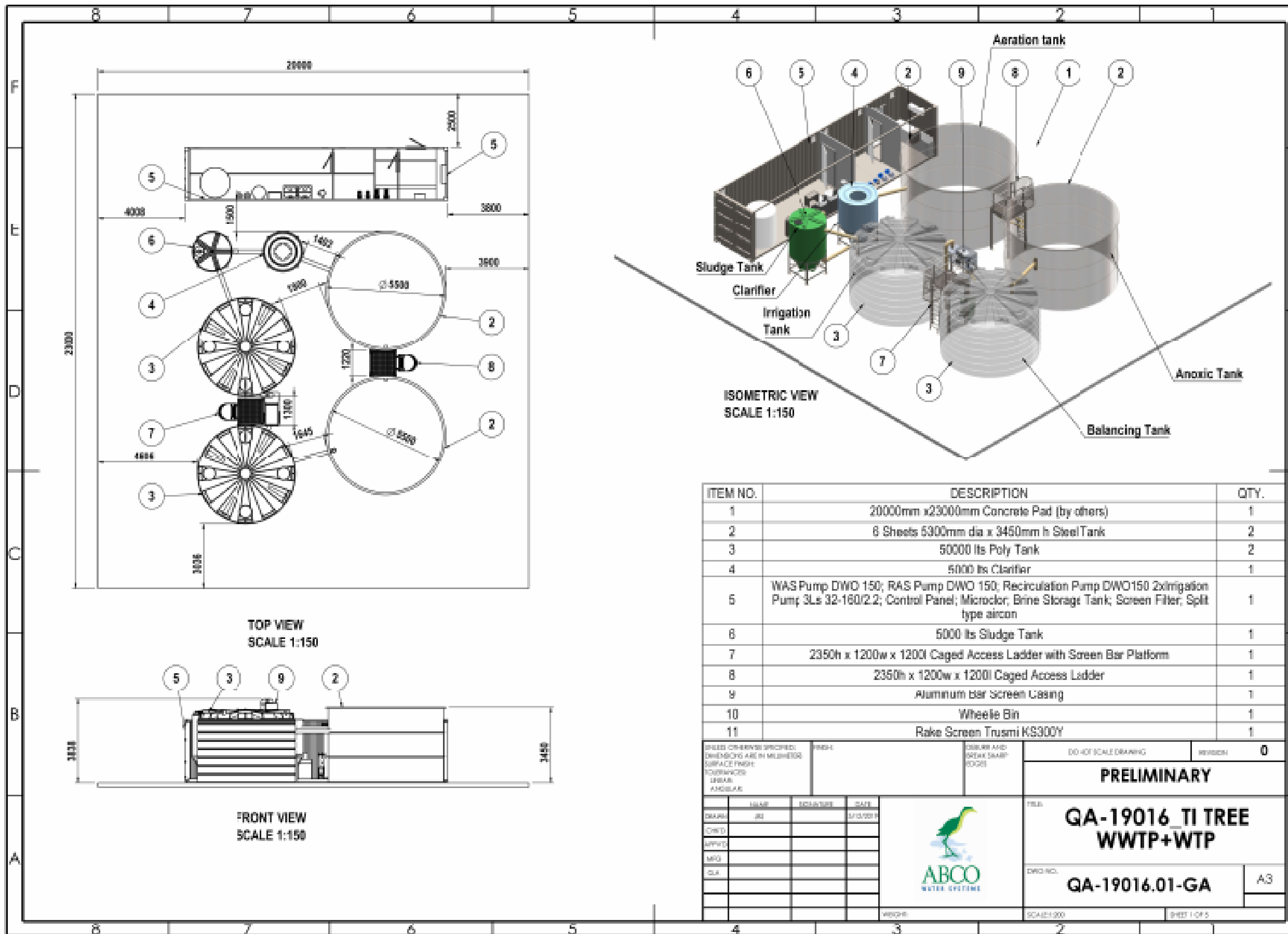
Figure 2: Wastewater treatment plant schematics
