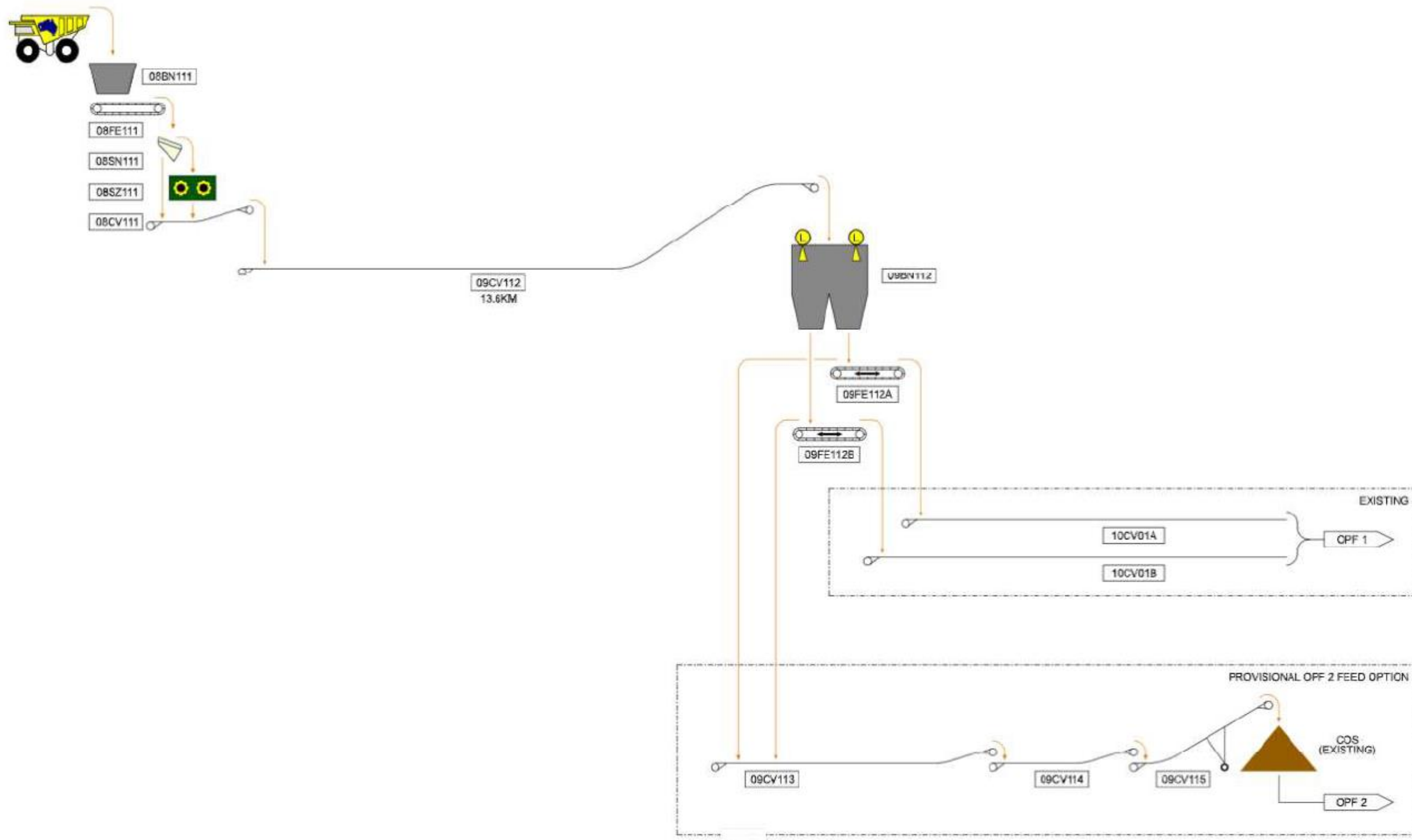
Figure 2: Proposed Hall Mining Hub Development Infrastructure and Process Flow Diagram
