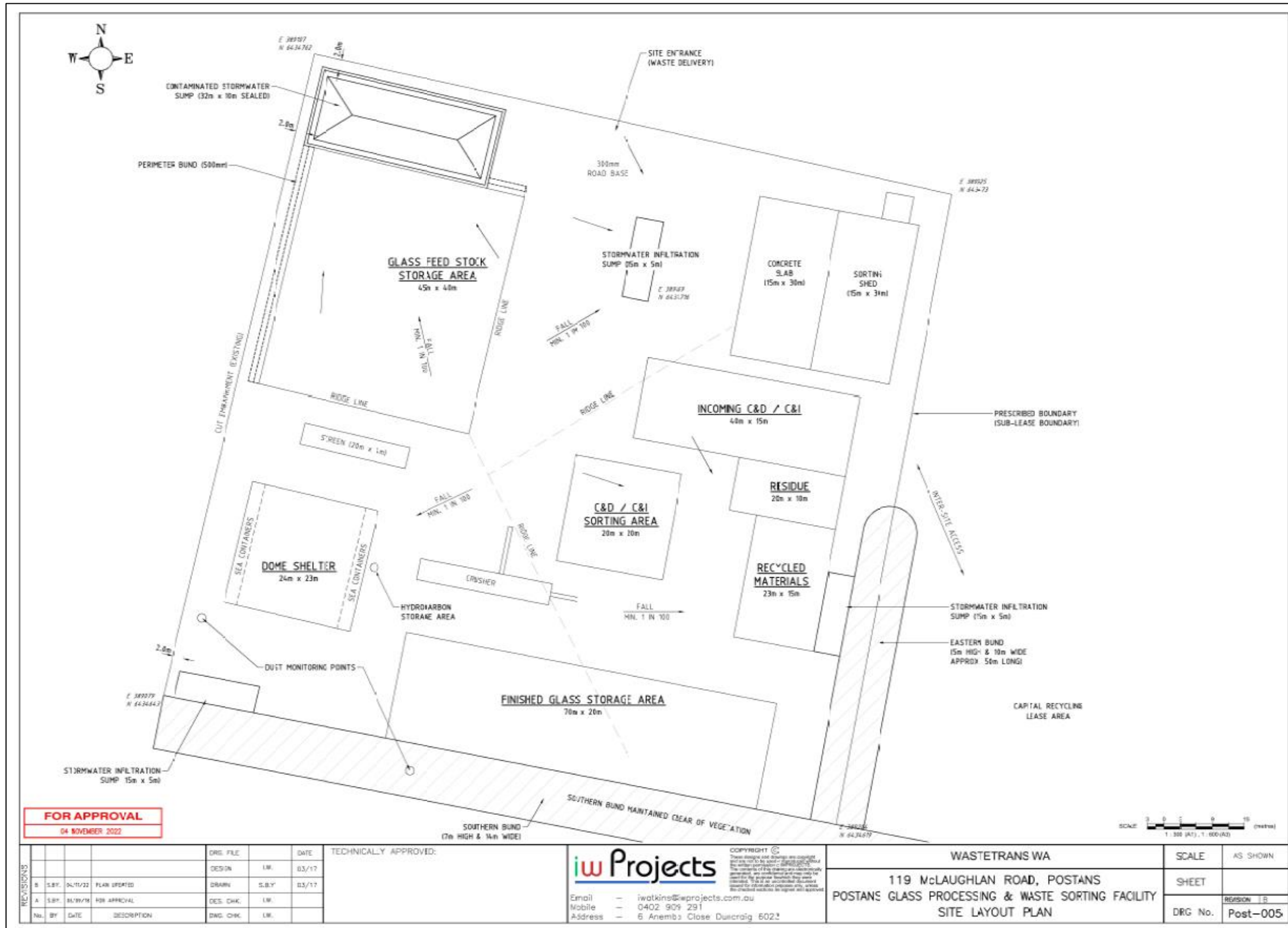
Figure 2: Layout of the Premises stormwater infiltration sumps, finished glass storage area, recycled materials stockpile, eastern and southern noise bunds, sorting shed, unprocessed glass stockpile, lined pond, contaminated stormwater sump and hydrocarbon storage area.
