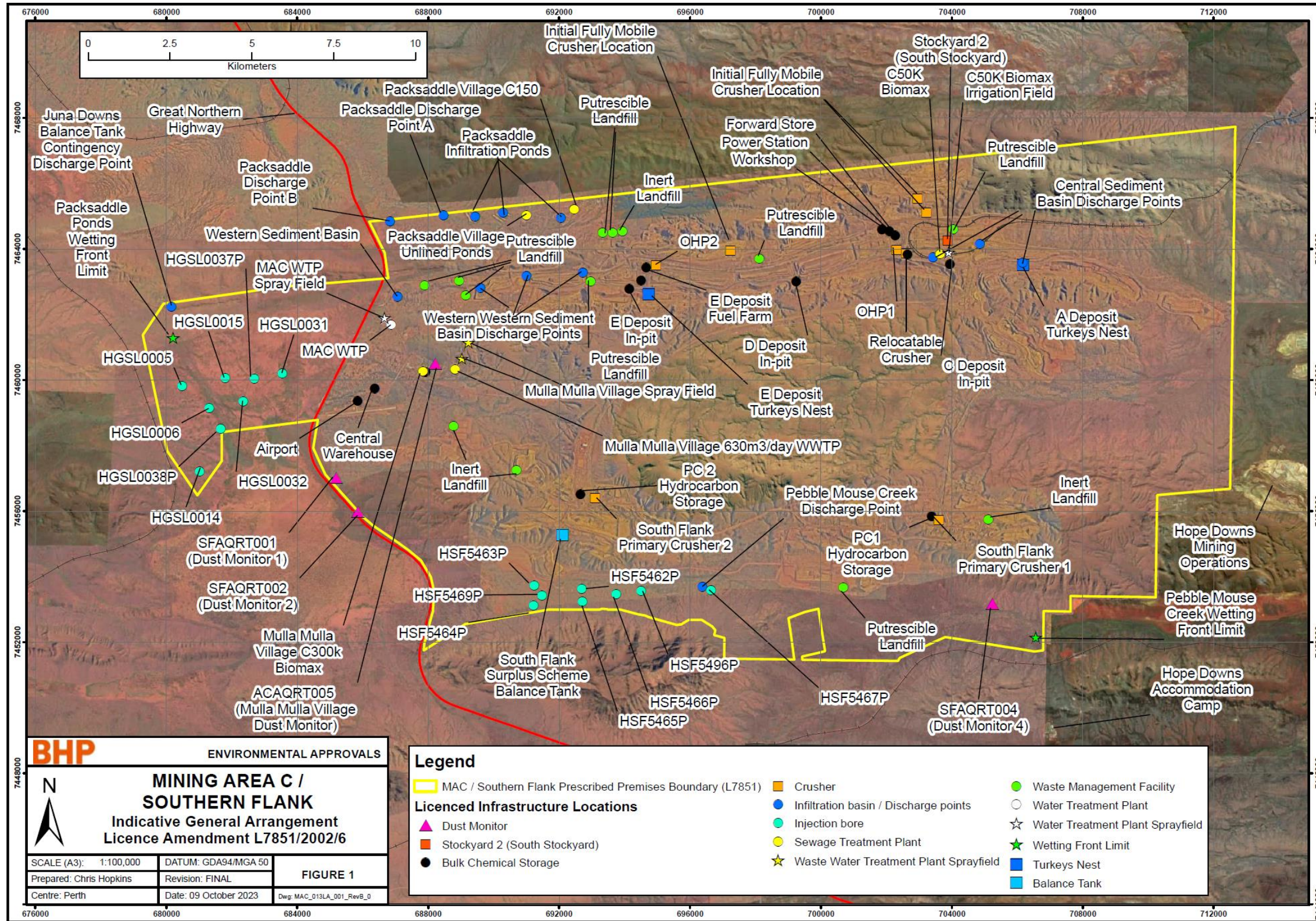
Figure 1: Site Layout and Prescribed Premises Boundary
