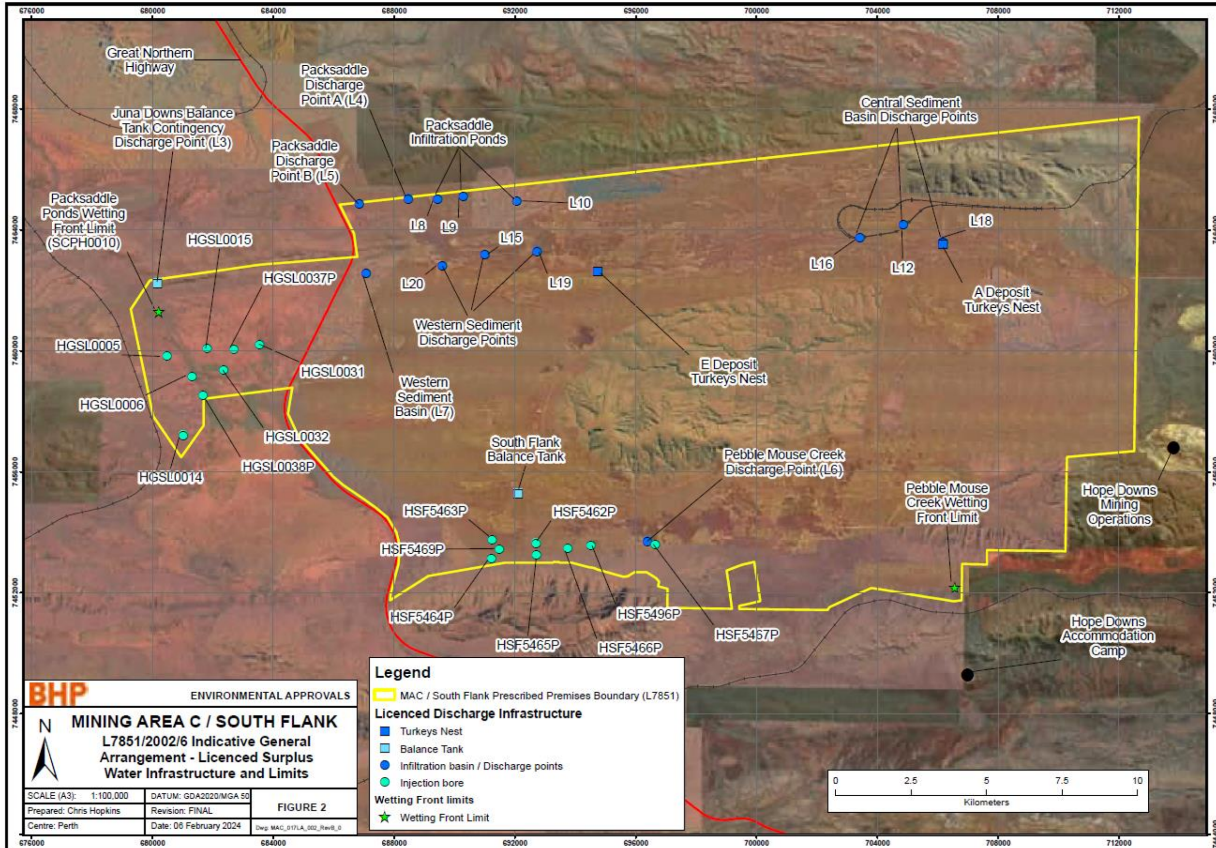
Figure 3: Site general arrangement of Licenced Surplus Water Infrastructure Wetting front limits
