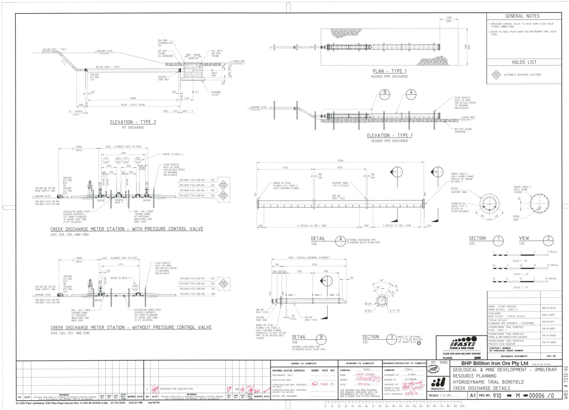
Figure 7: BHP's Standard Discharge Point Design
