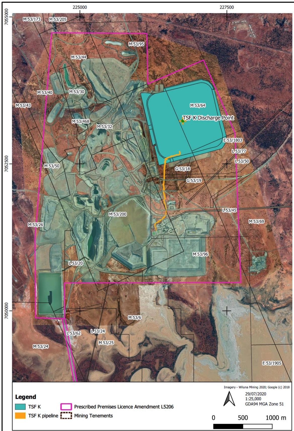
Figure 3: Locations of pipeline connecting TSF K to the CIL Plant
