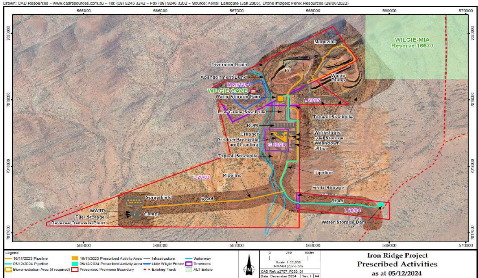
Figure 2: Prescribed activities and new water storage dam
