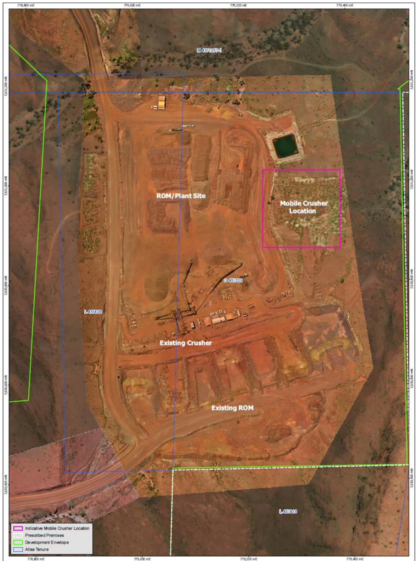
Figure 6: Location of the proposed secondary crushing and screening facility
