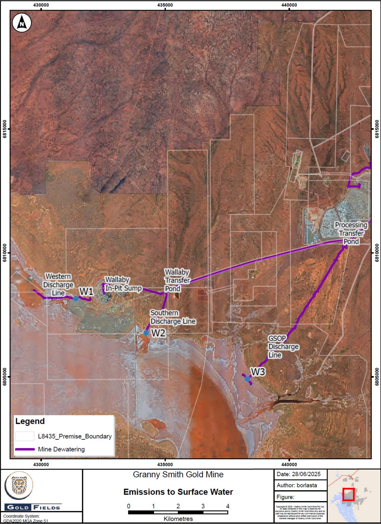
Figure 9: Emission and monitoring locations for W1, W2 and W3
