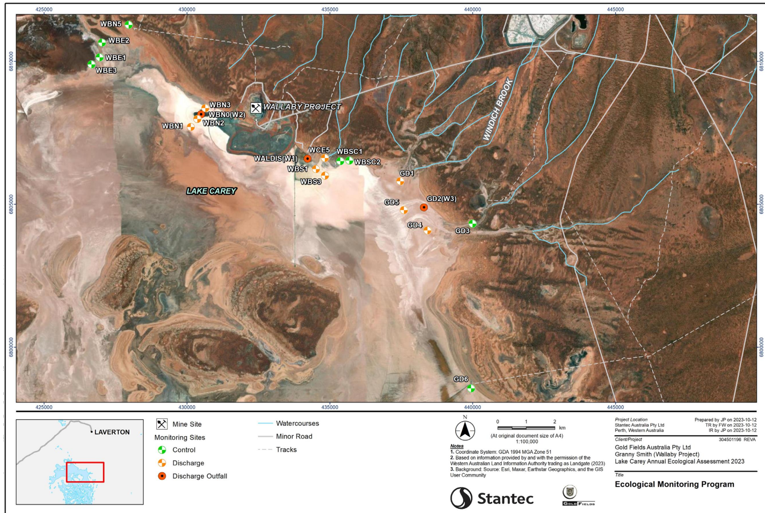
Figure 16 Location of Annual Ecological Assessment monitoring sites for the W1, W2 and W3 discharge outfalls
