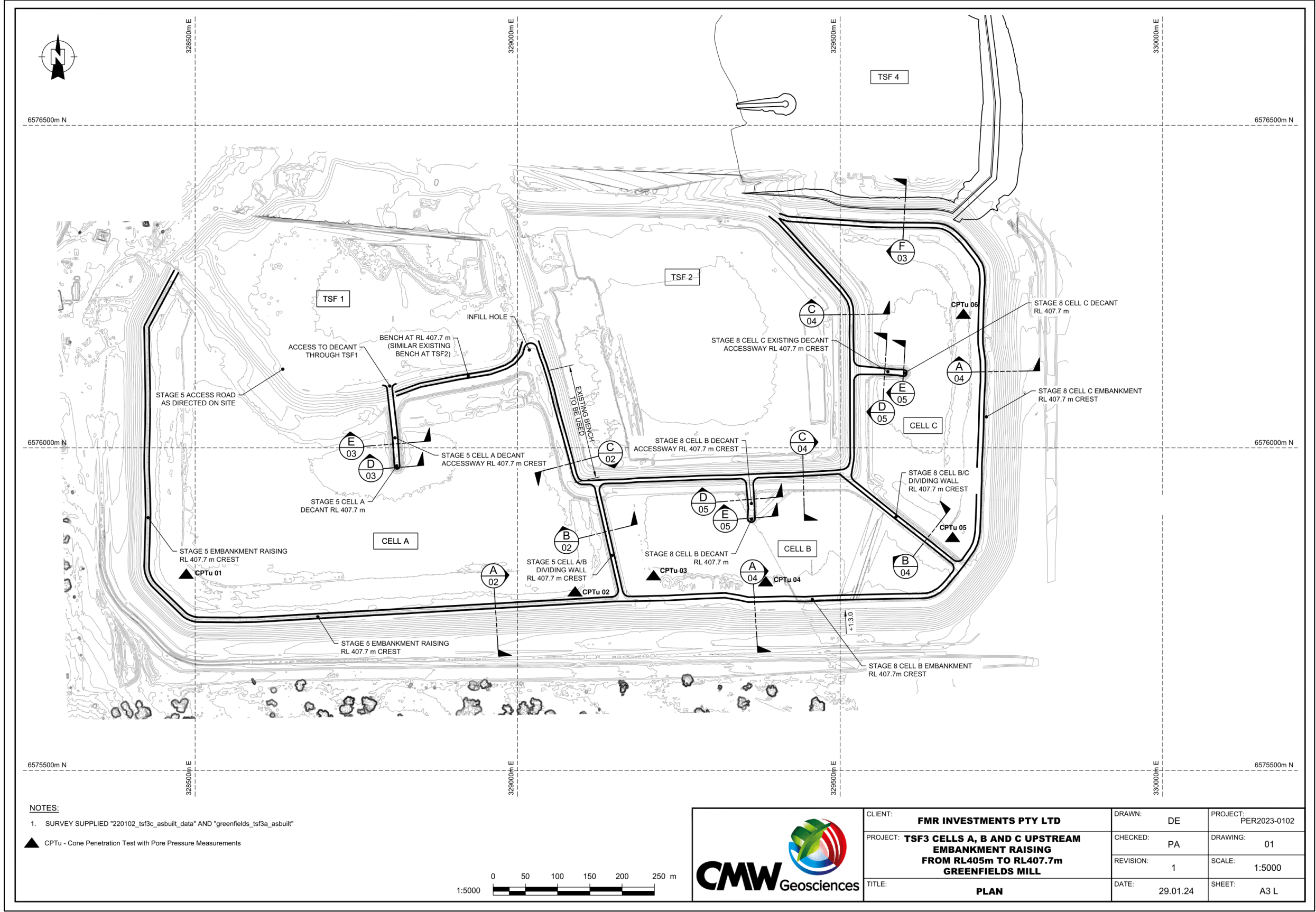
Figure 2: Design drawing for TSF3 Cell A (Stage 5), Cell B (Stage 8), and Cell C (Stage 8) embankment raise to RL 407.7 m
