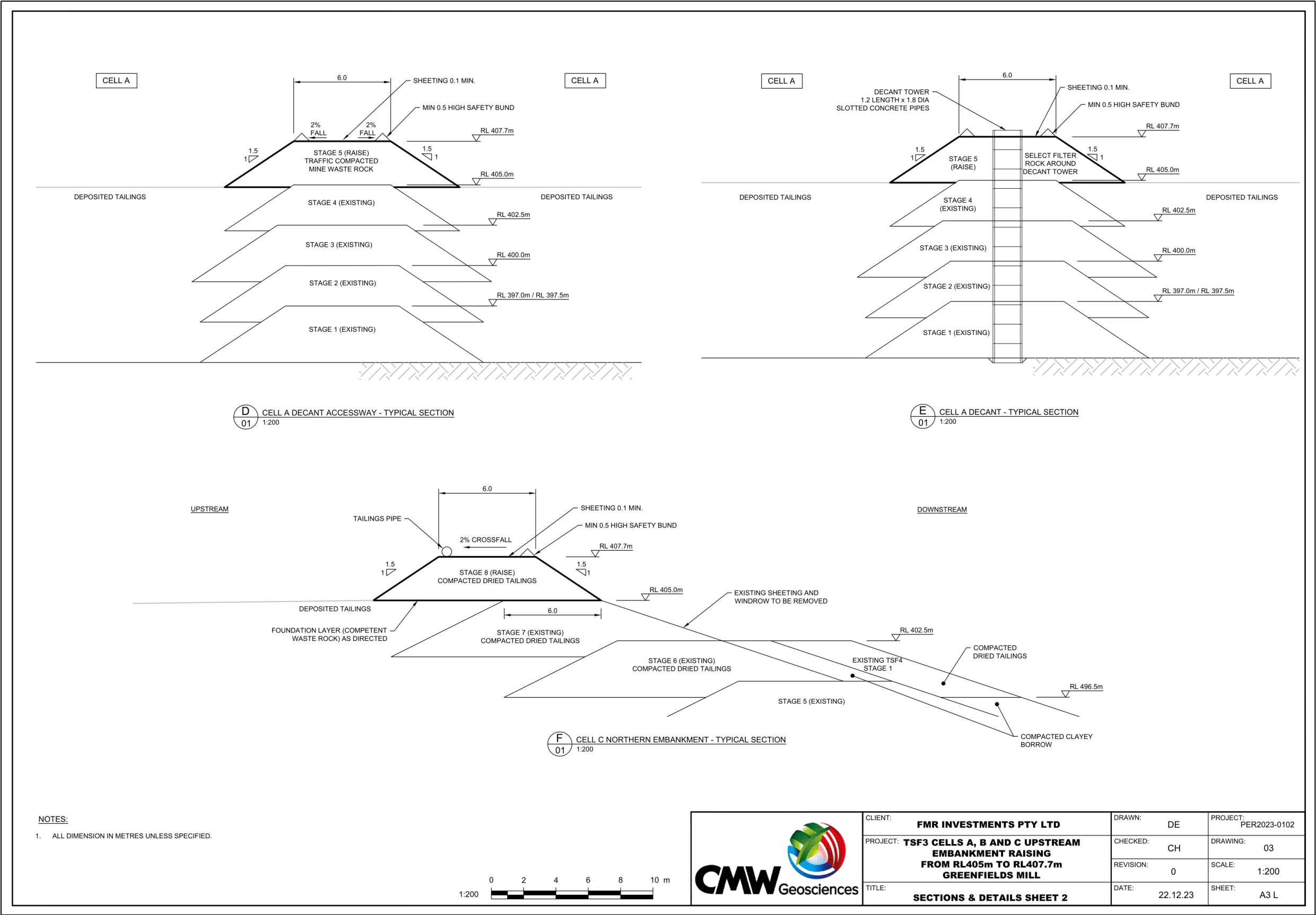
Figure 4: Design drawing (cross-section) for TSF3 Cell A Stage 5 embankment raise – decant structure and accessway and Cell C Stage 8 northern embankment raise
