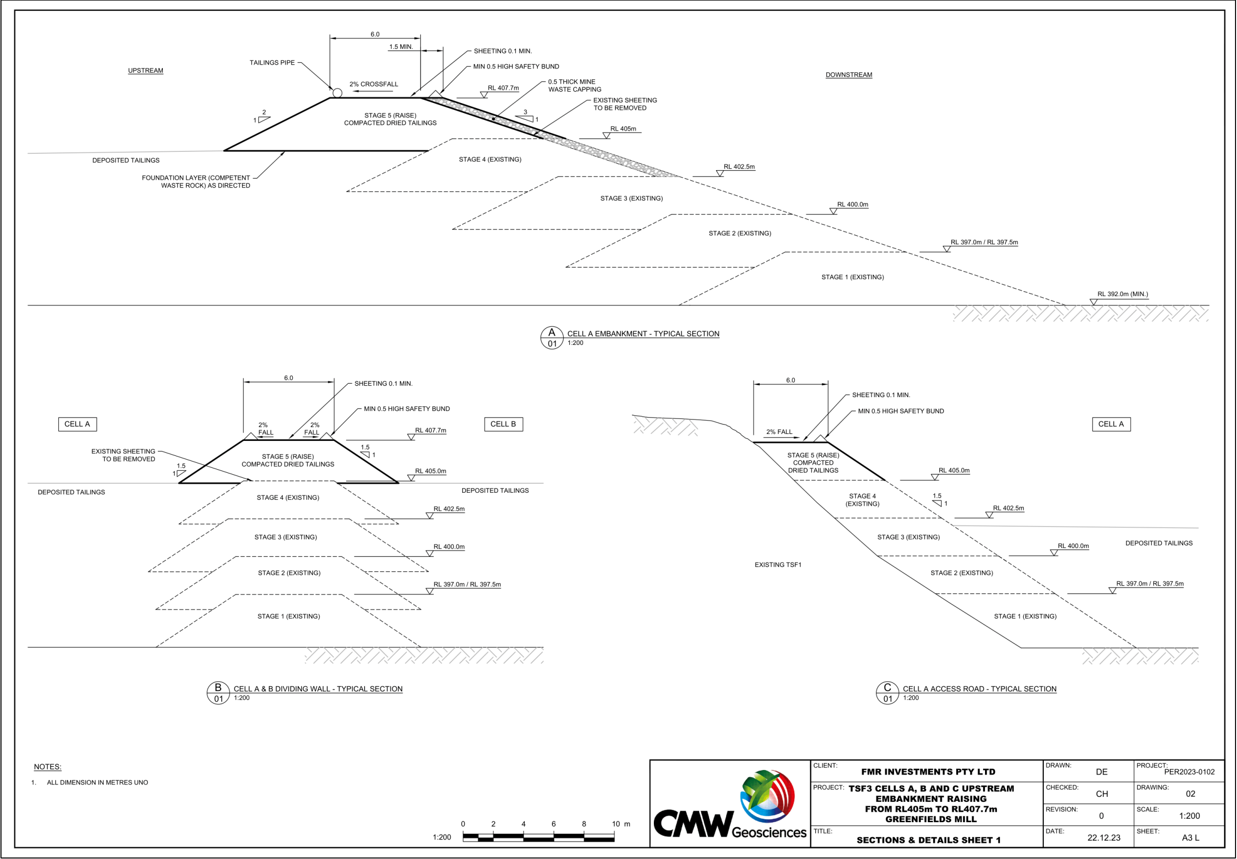
Figure 3: Design drawing (cross-section) for TSF3 Cell A Stage 5 embankment raise
