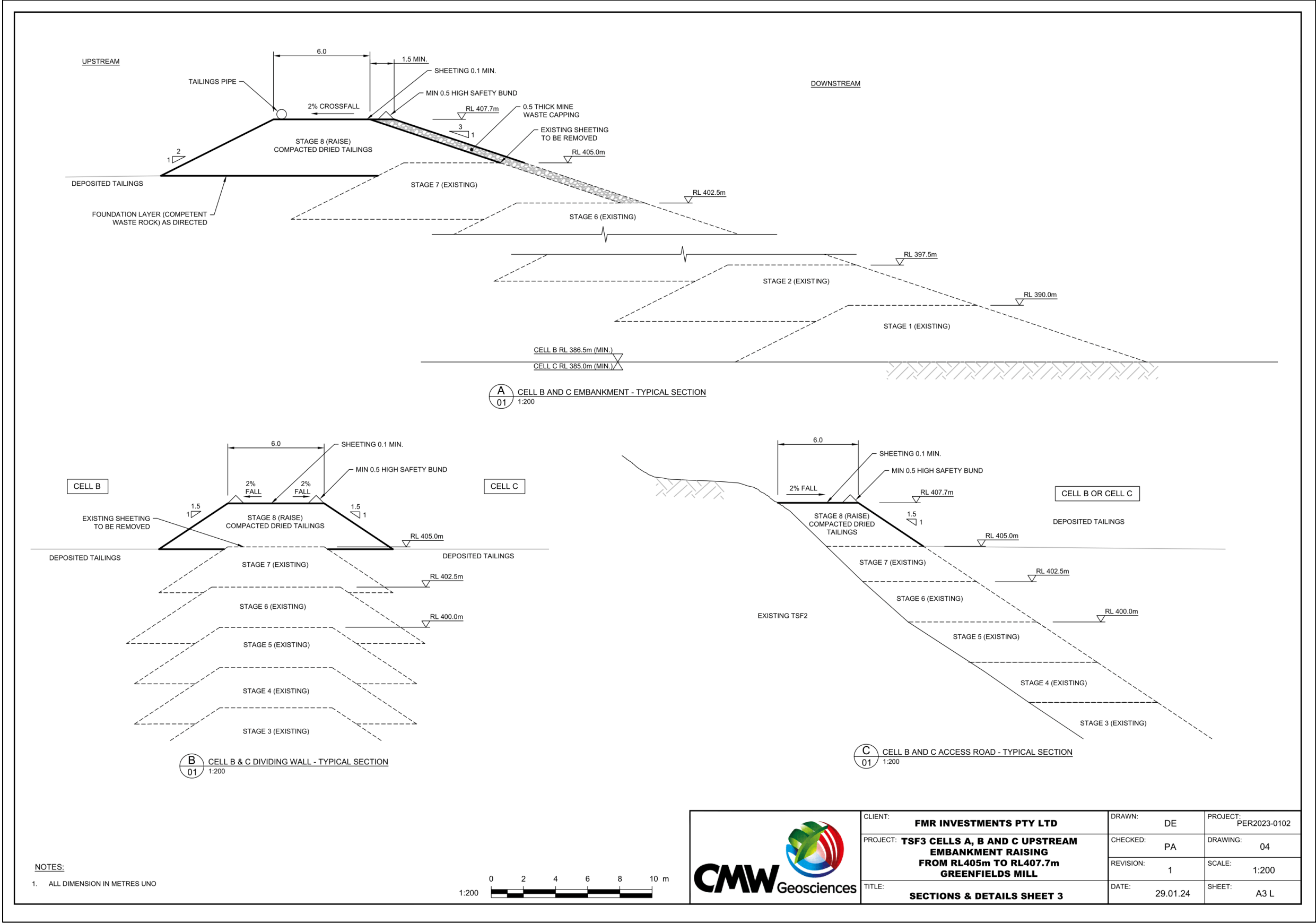
Figure 5: Design drawing (cross-section) for TSF3 Cell B and Cell C Stage 8 embankment raise
