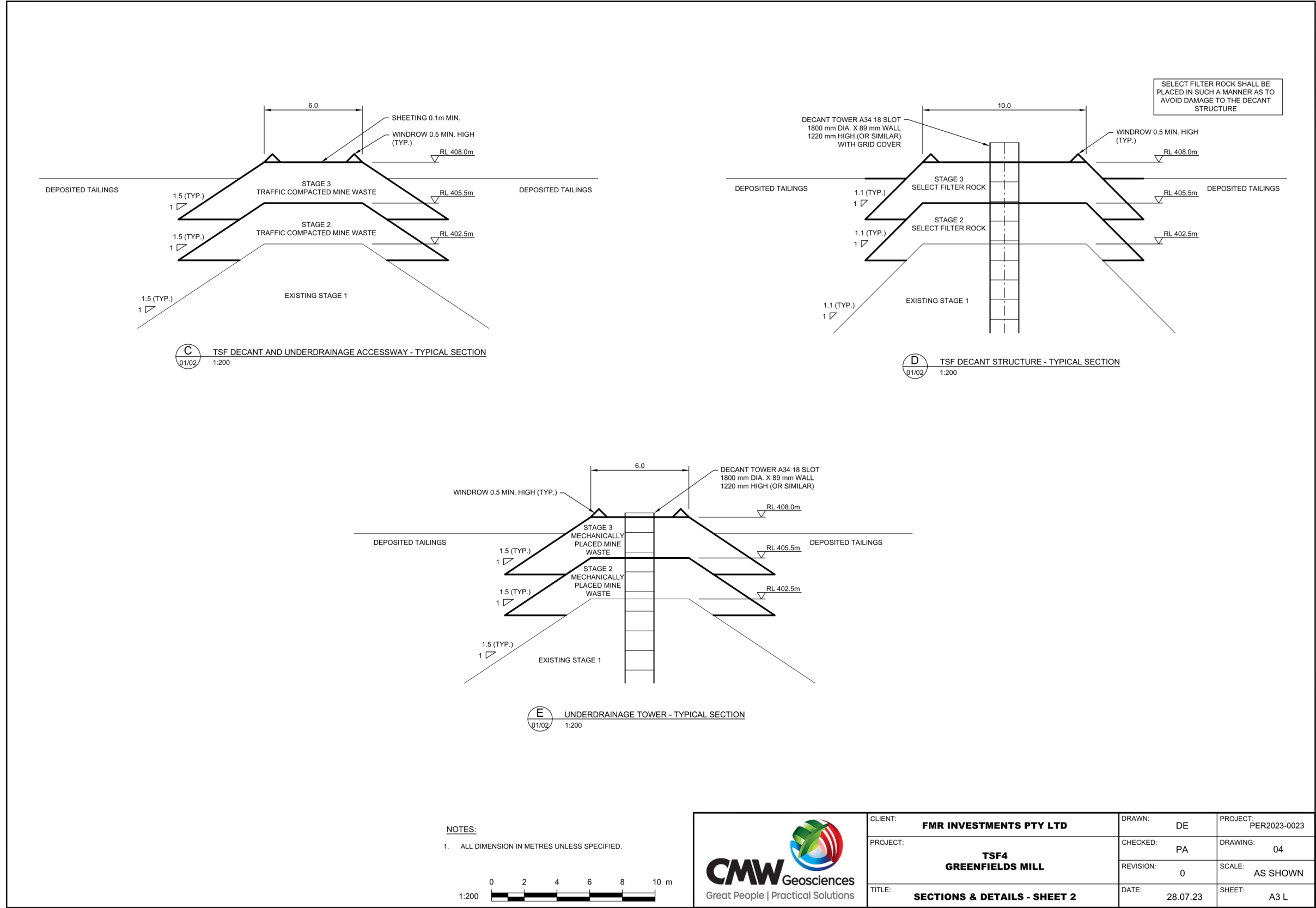
Figure 1: Design drawing for TSF4 Stage 2 and 3 embankment raises – decant structure, underdrainage tower and accessway
