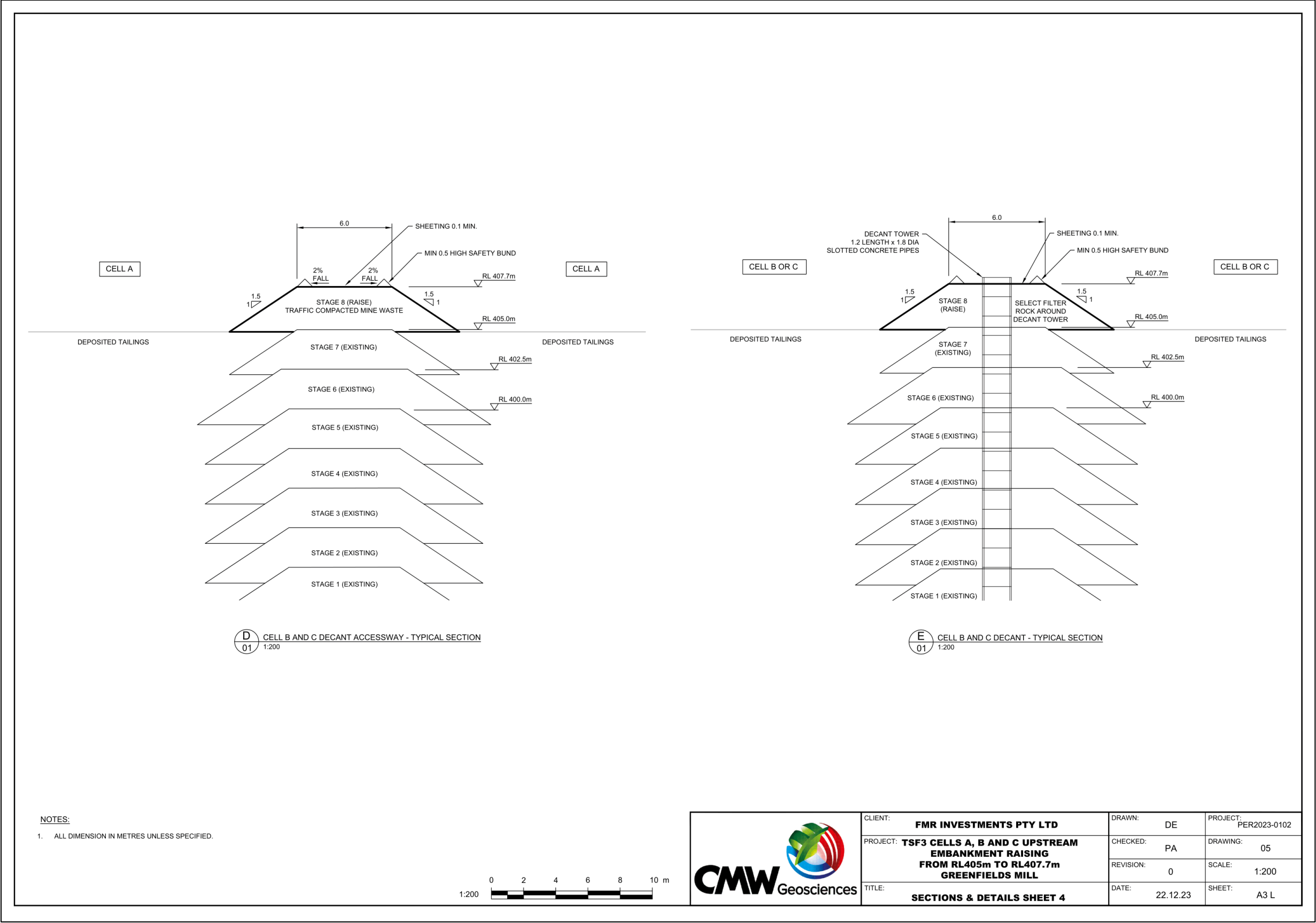
Figure 6: Design drawing (cross-section) for TSF3 Cell B and Cell C Stage 8 embankment raise – decant structure and accessway
