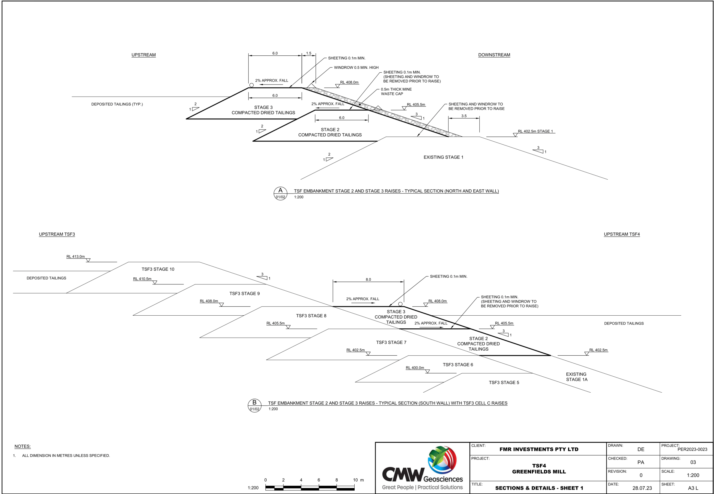
Figure 9: Design drawing (cross-section) for TSF4 Stage 2 and 3 embankment raises
