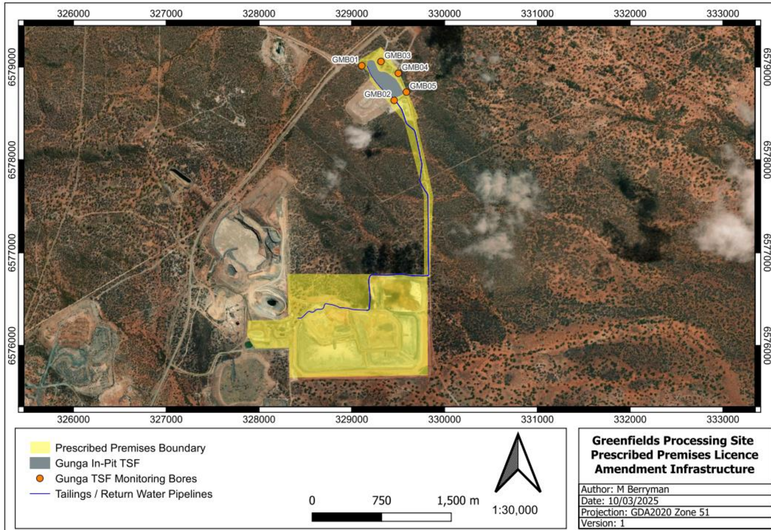
Figure 6: Greenfields Processing Site's Tailings/return Water Pipelines
