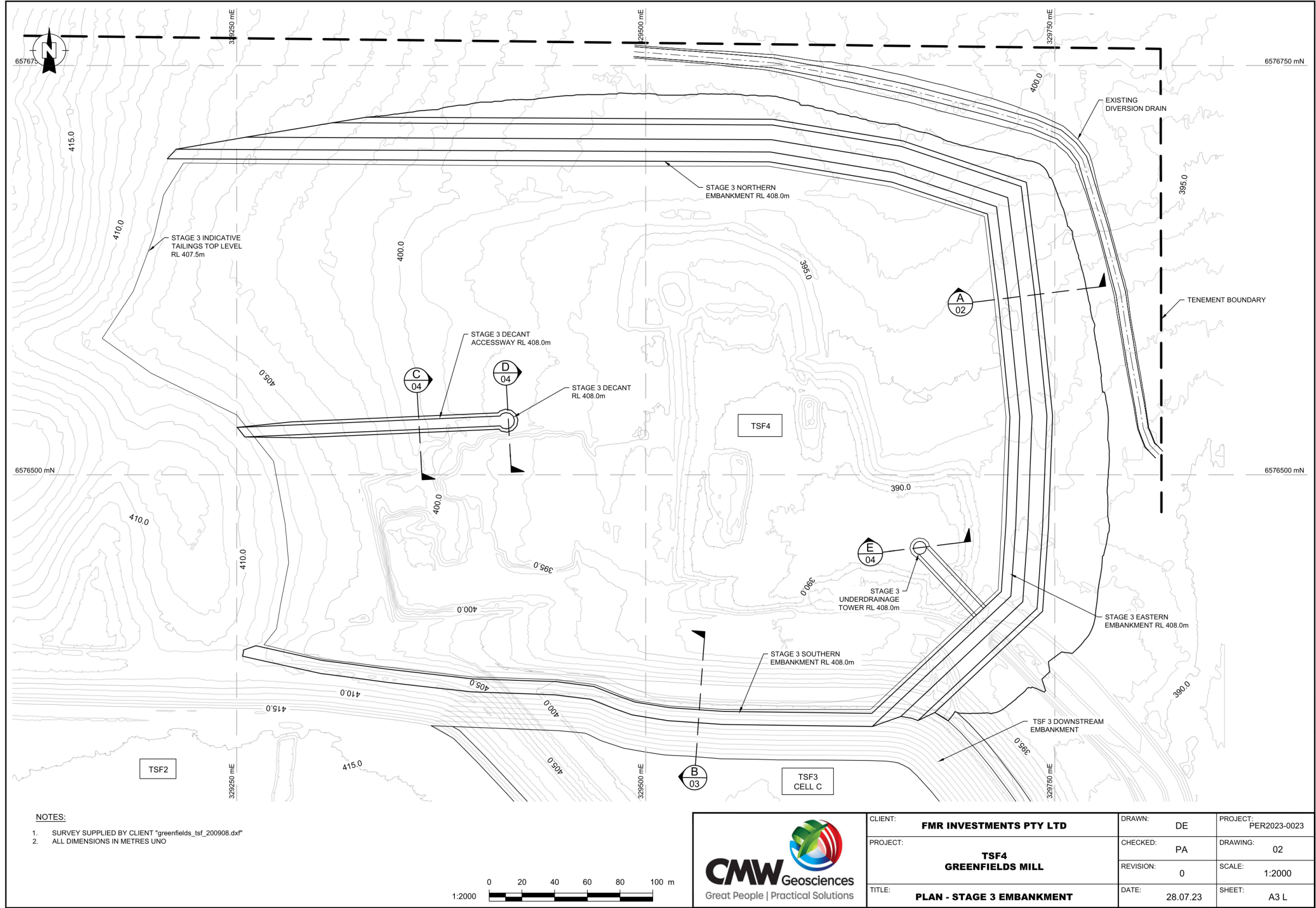
Figure 8: Design drawing for TSF4 Stage 3 embankment raise
