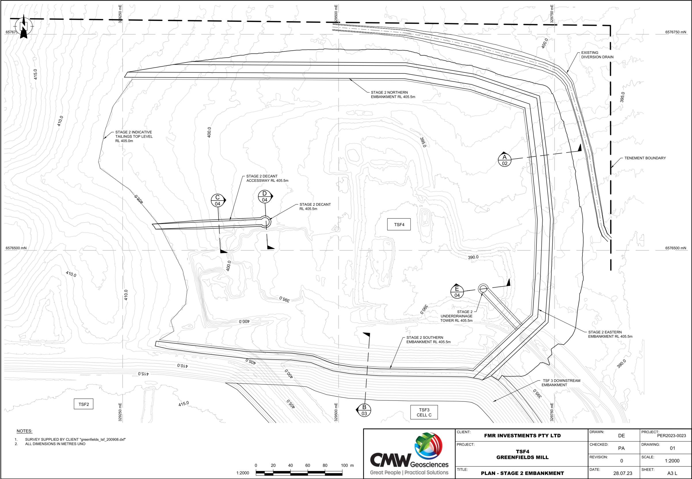
Figure 7: Design drawing for TSF4 Stage 2 embankment raise
