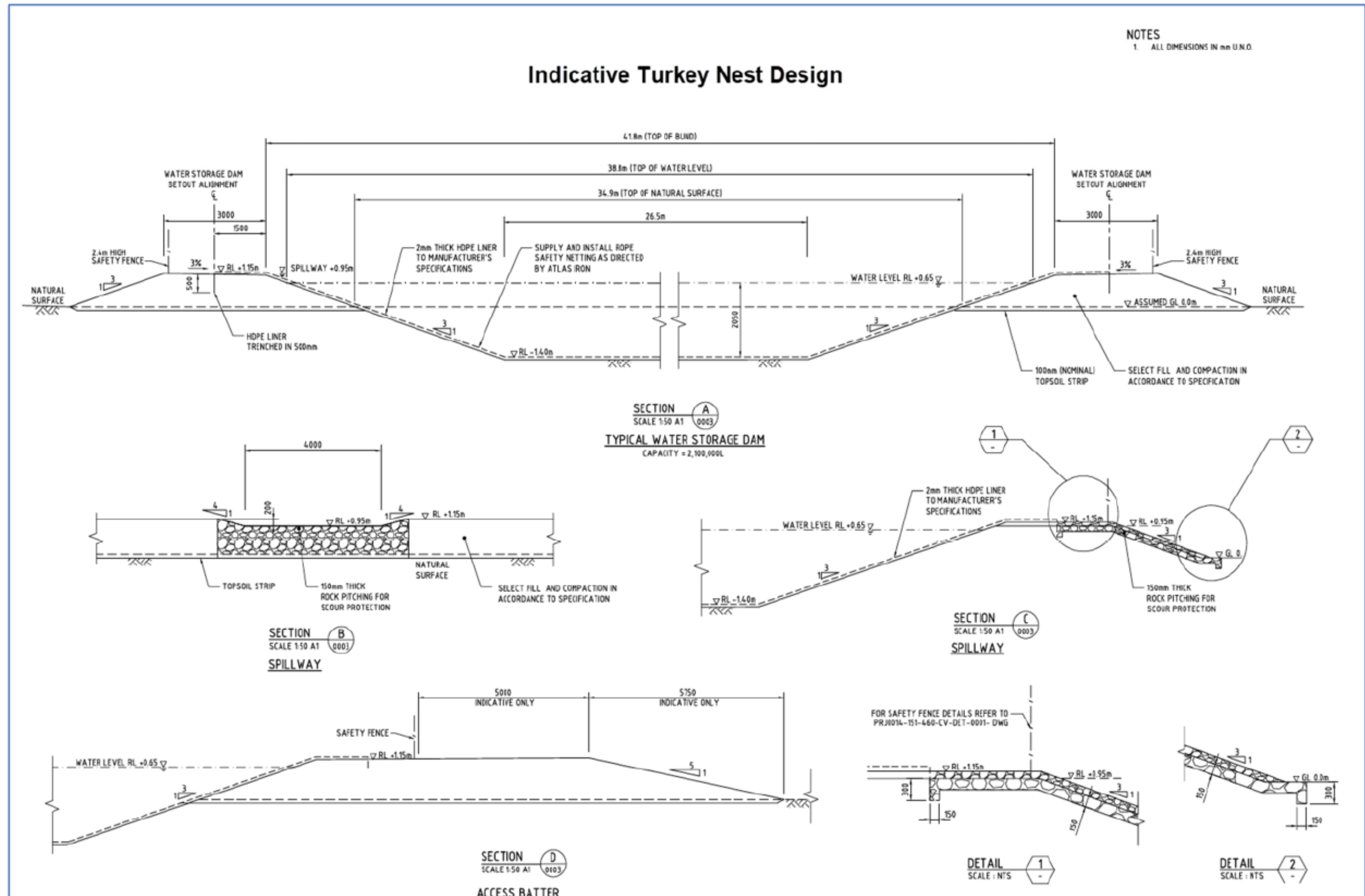
Figure 15: Indicative turkey's nest design
