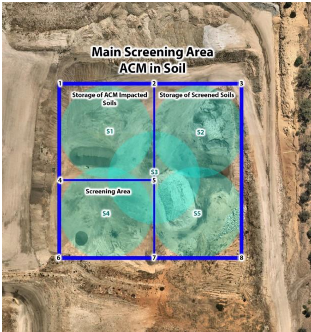
Figure 3: Detailed view of Main Screening Area and layout of dust suppression sprinklers
