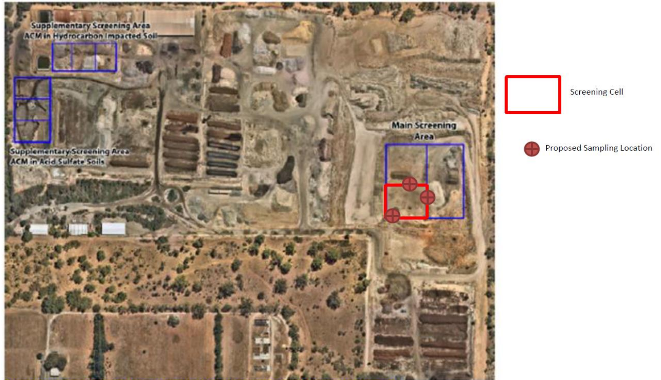
Figure 5: Indicative asbestos fibre monitor locations under a south-westerly wind direction scenario for screening activities within the Main Screening Area
