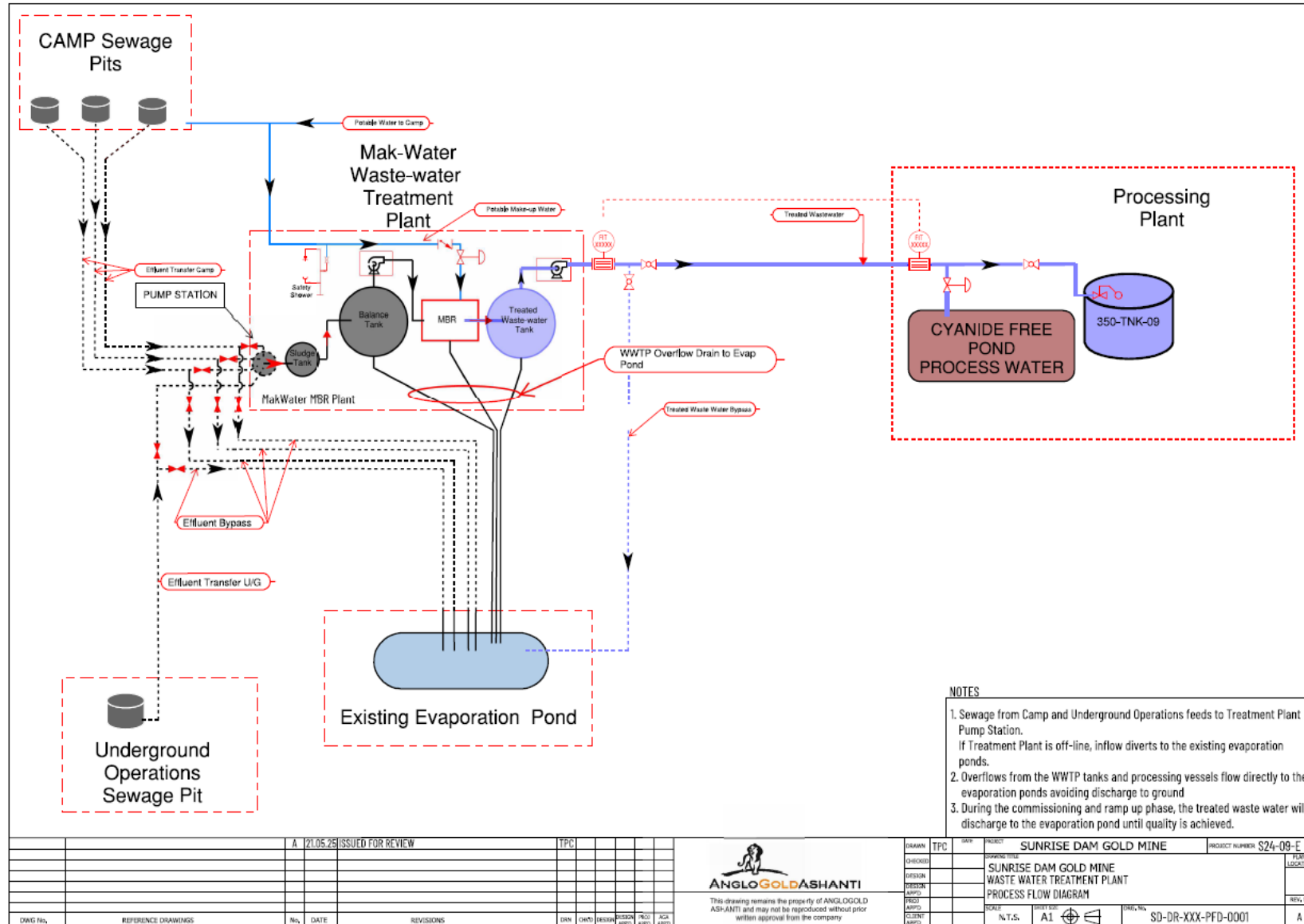
Figure 9: Sewage water process diagram
