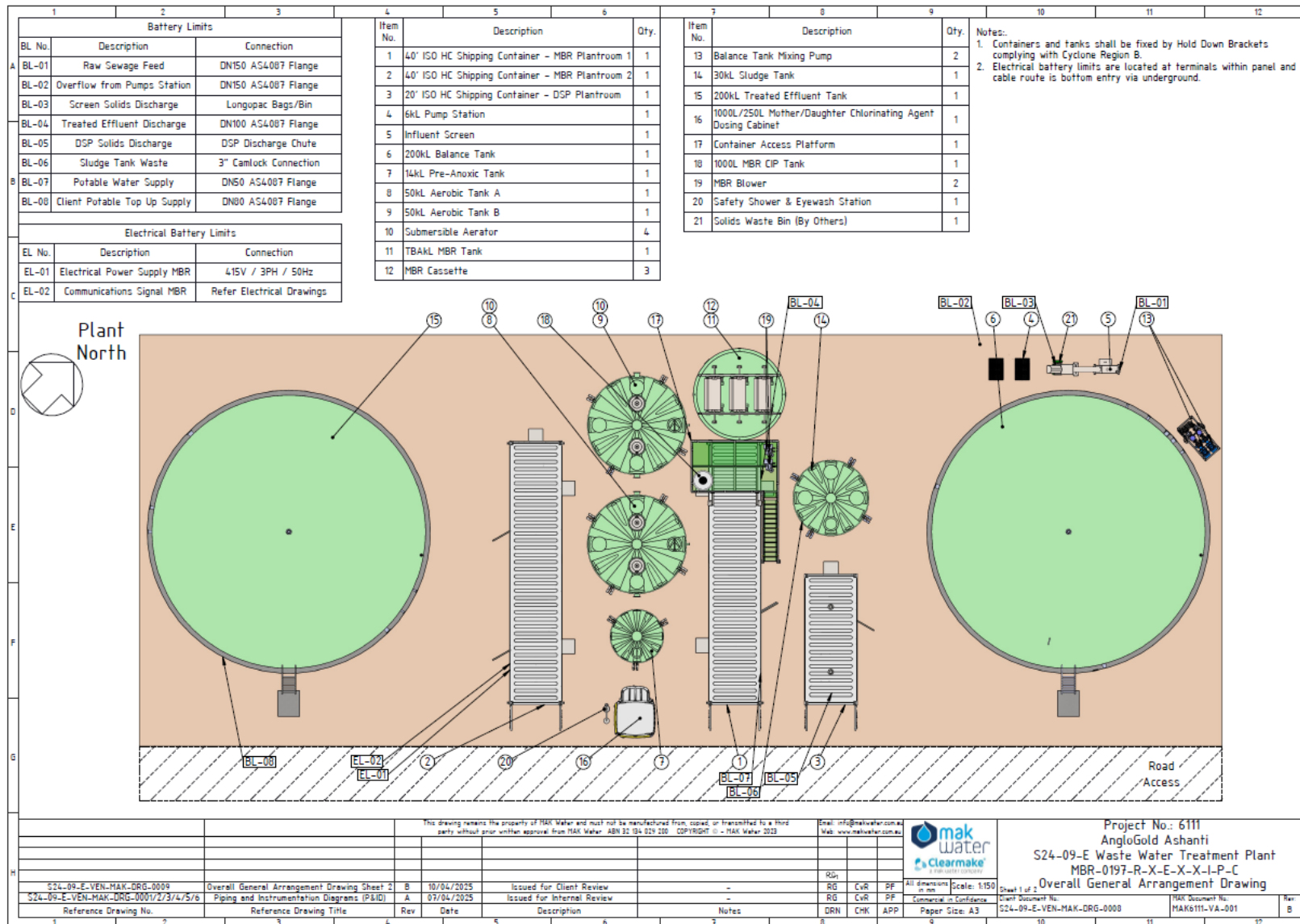
Figure 8: MBR treatment plant design
