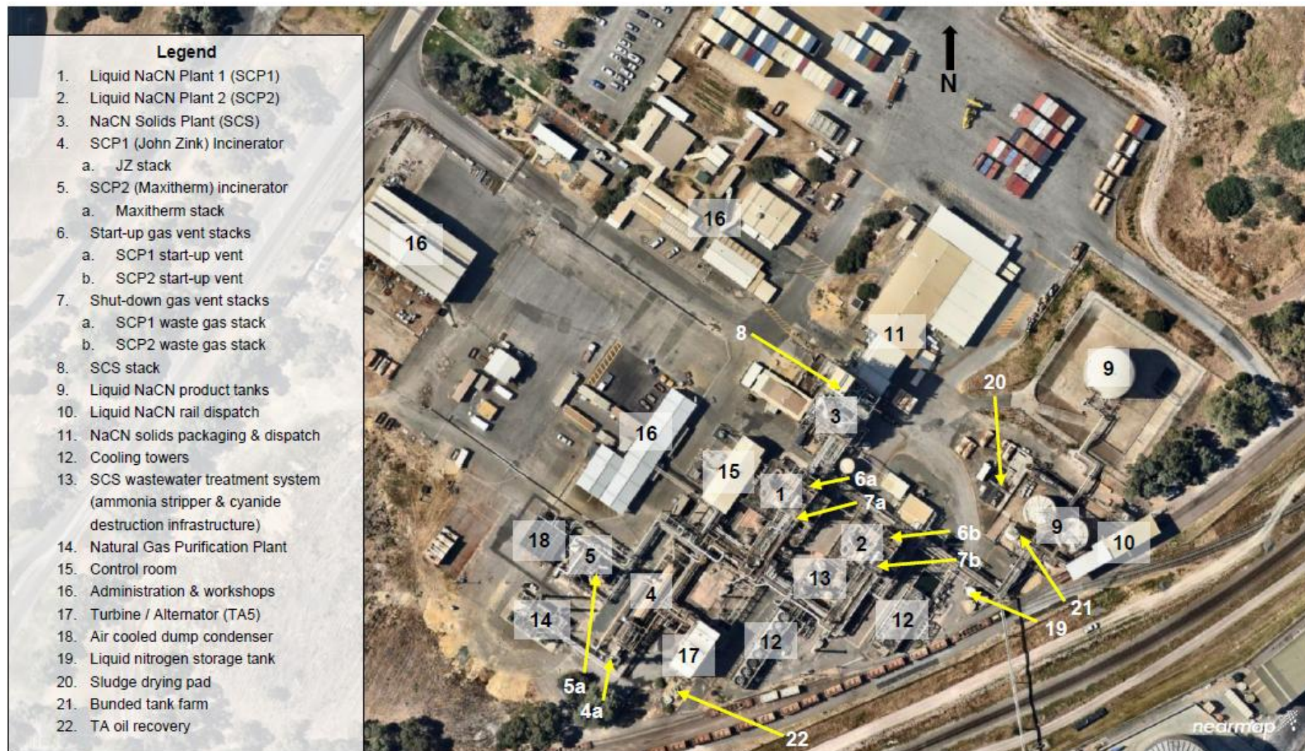
Figure 2: General layout of Sodium Cyanide Manufacturing Facility
