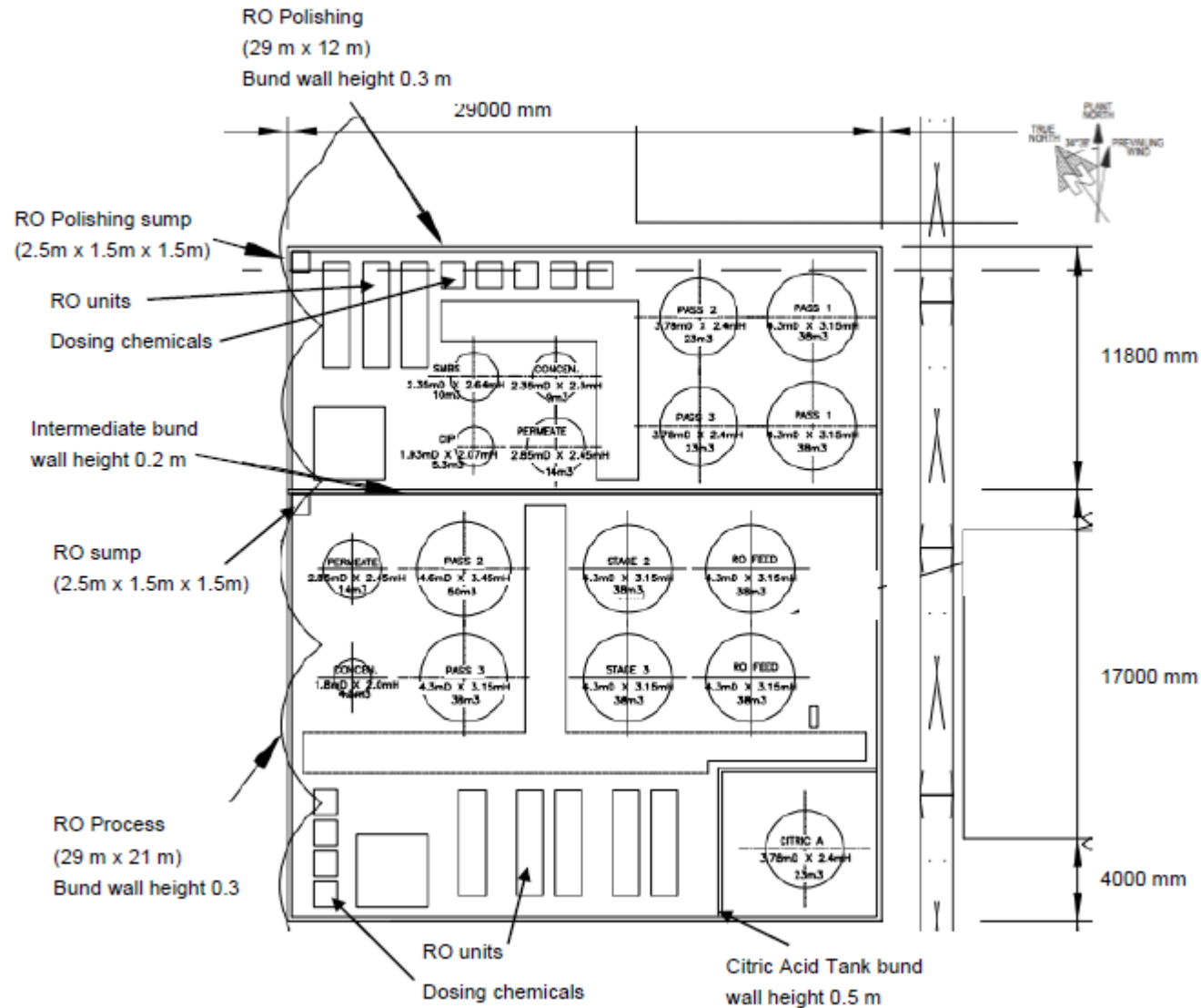
Figure 6: Process RO and Polishing RO treatment plant layout
