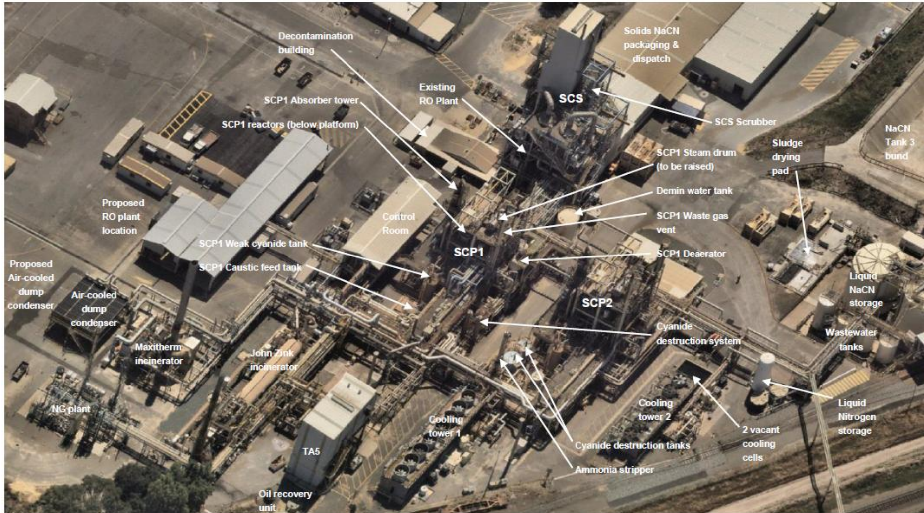
Figure 3: Sodium Cyanide Plant key component identification
