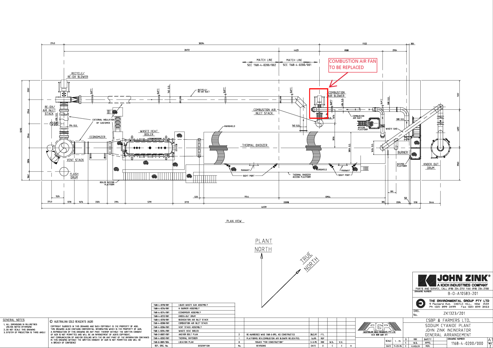
Figure 8: Location of combustion air fan within John Zink incinerator.
