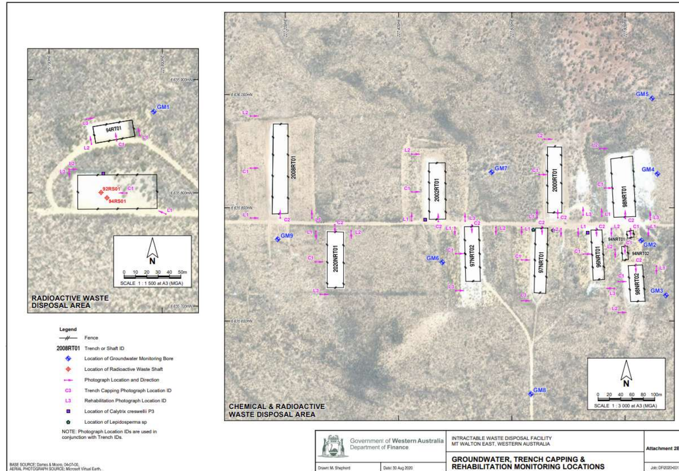
Figure 2: Groundwater monitoring locations
