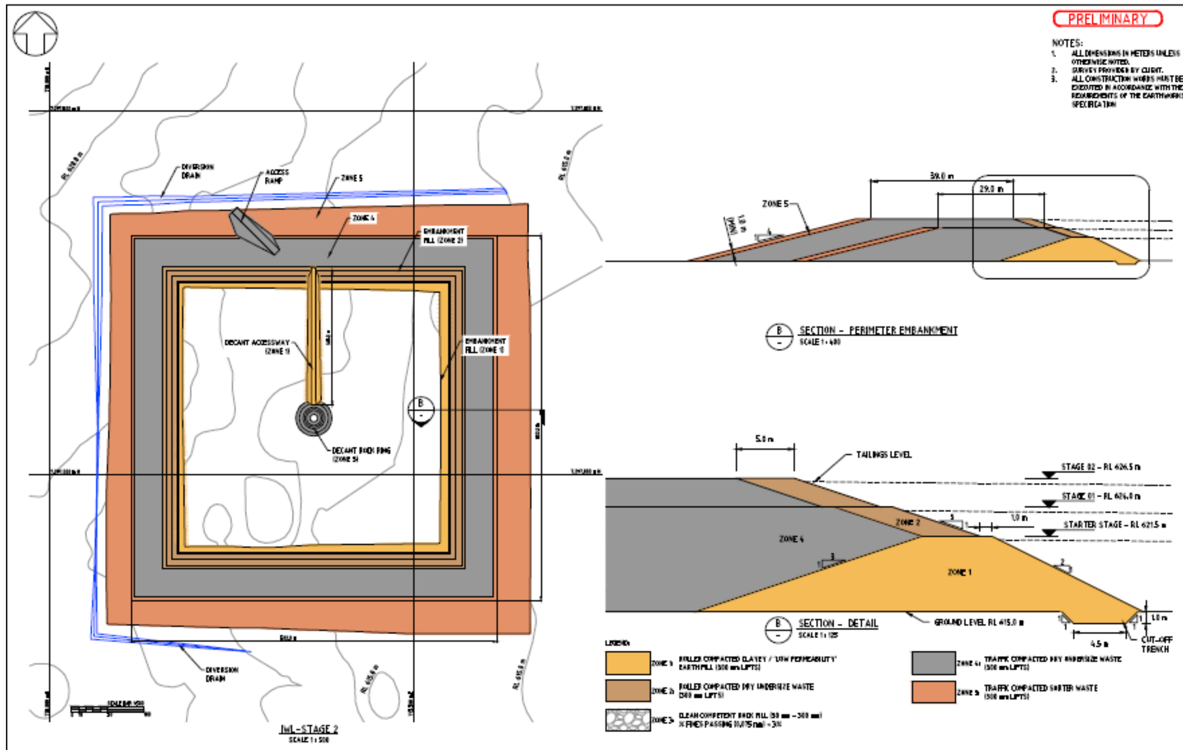
Figure 6: Stage 2 lift Plan and embankment sections
