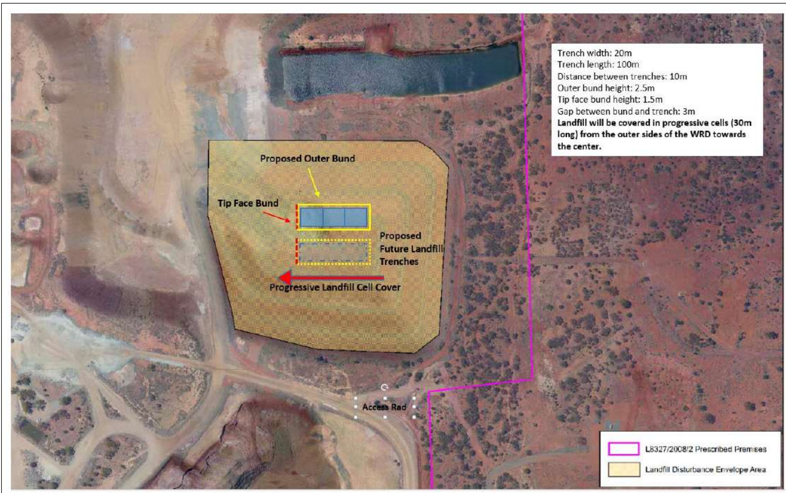
Figure 2: Design of Landfill Facility
