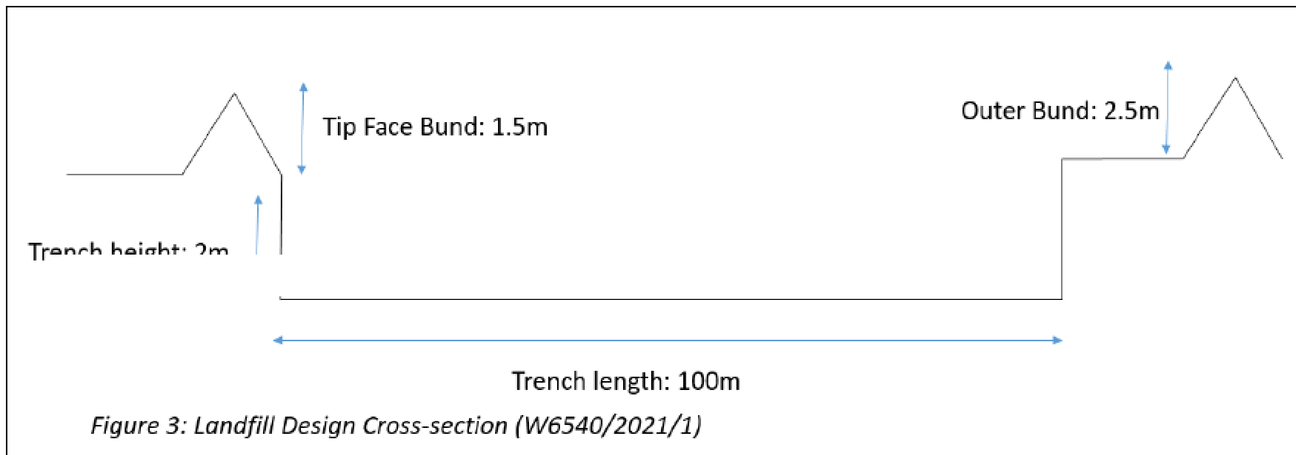
Figure 3: Landfill Design Cross-Section
